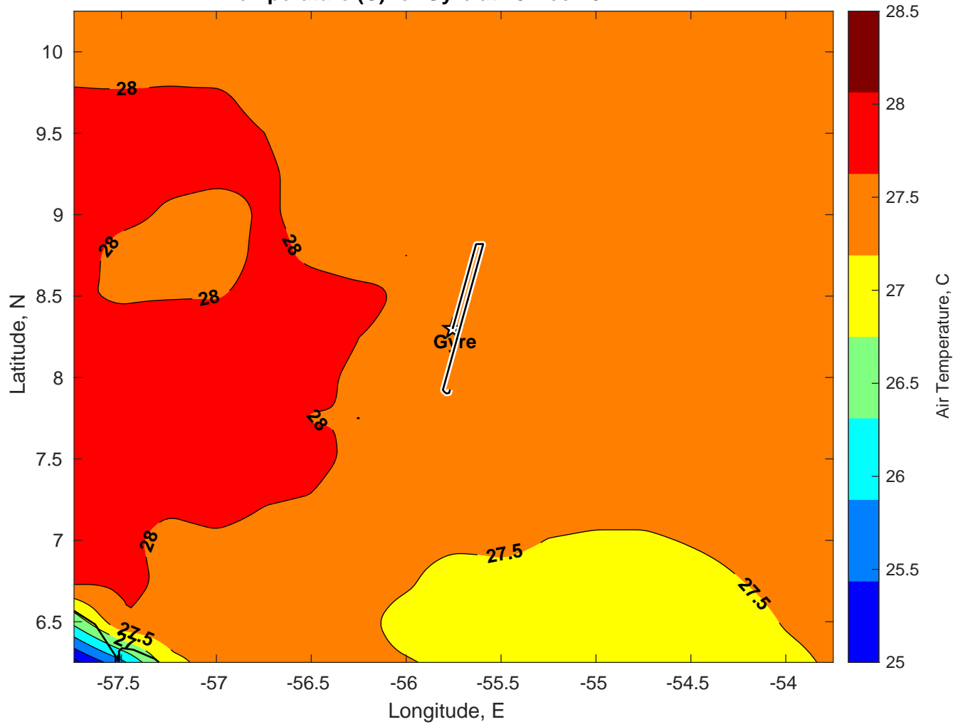
Air Temperature (C) for Gyre at 28-Dec-2024
