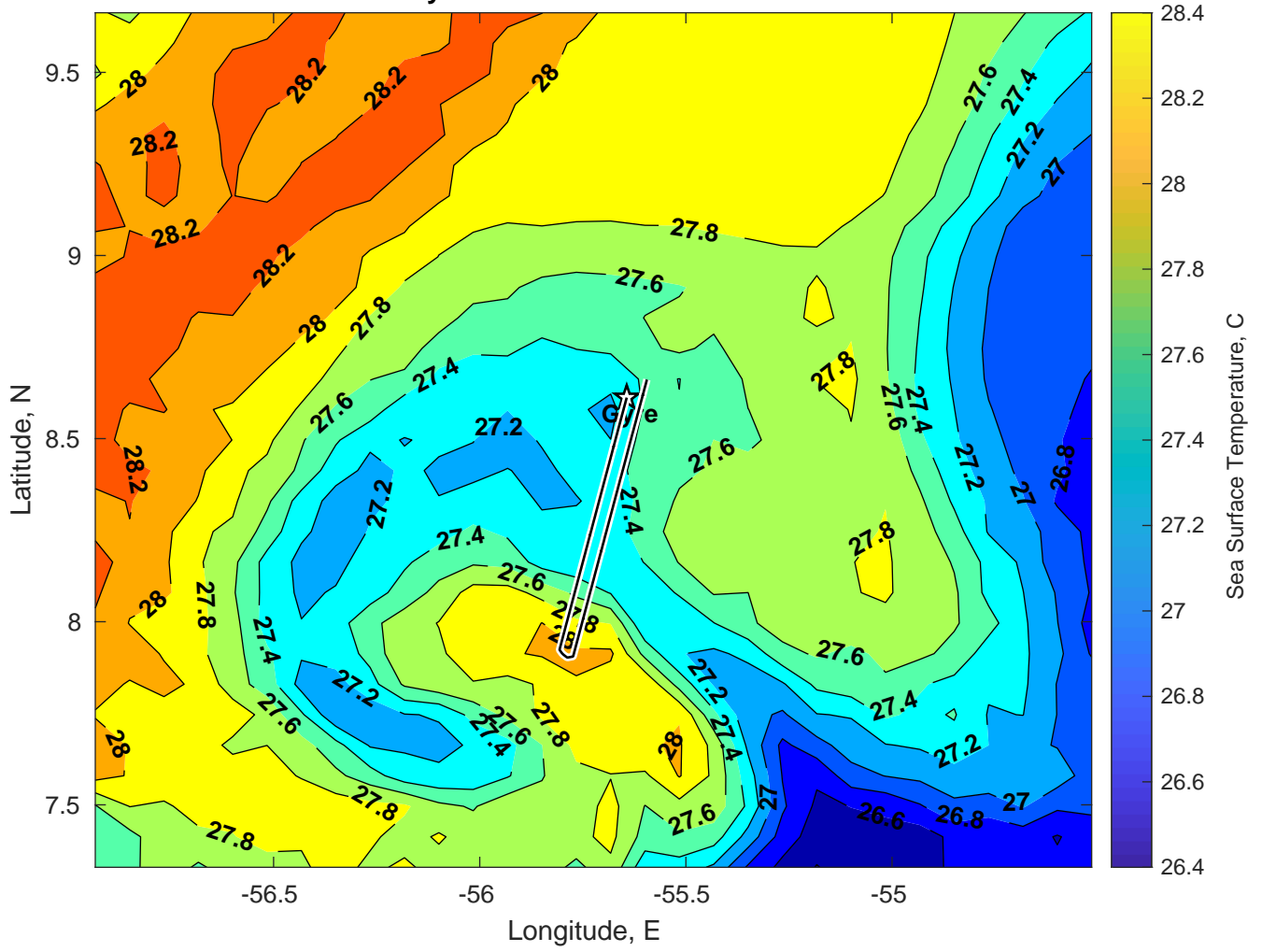
SST for Gyre at 27-Dec-2024 00:00:00
