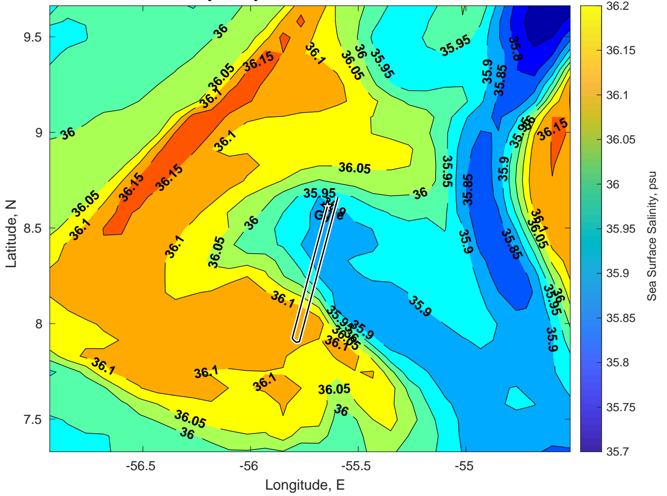
Surface Salinity for Gyre at 27-Dec-2024 00:00:00
