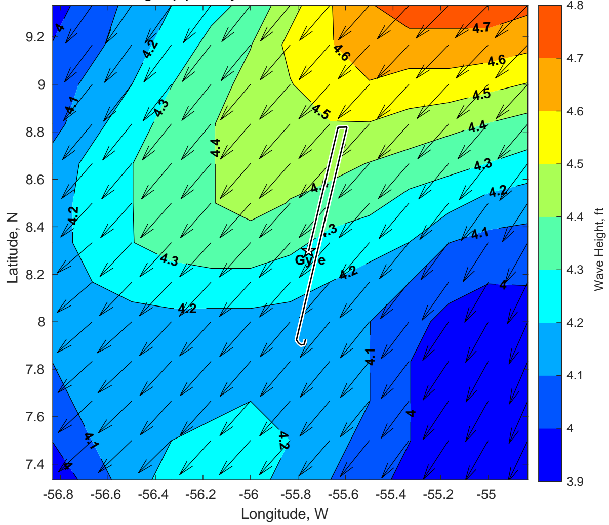
Wave Height (ft) for Gyre at 28-Dec-2024 09:00:00
