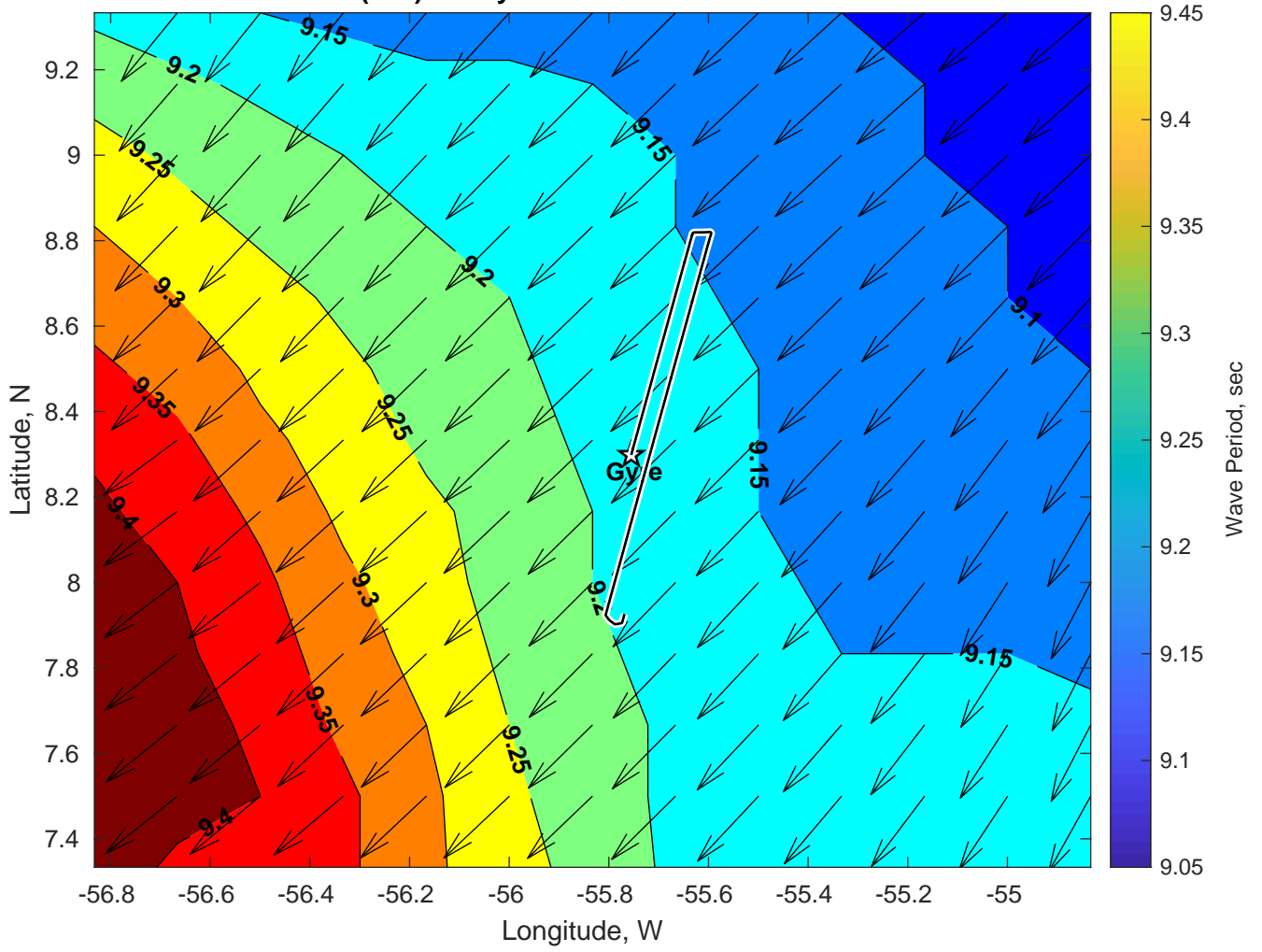
Wave Period (sec) for Gyre at 28-Dec-2024 09:00:00
