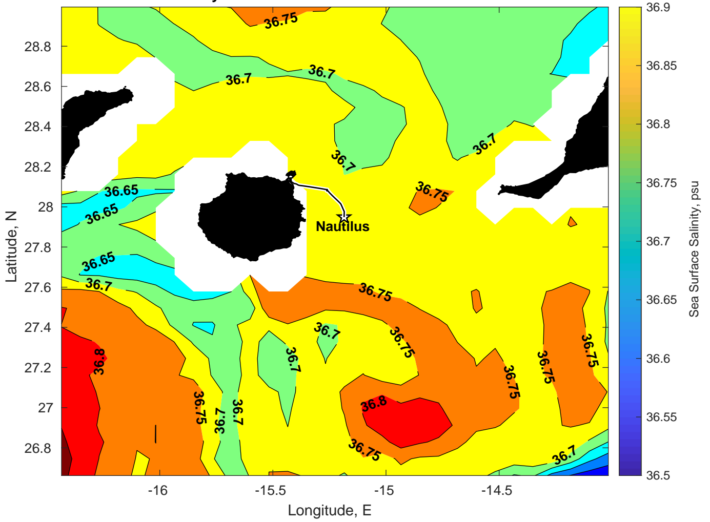
Surface Salinity for Nautilus at 27-Dec-2024 00:00:00
