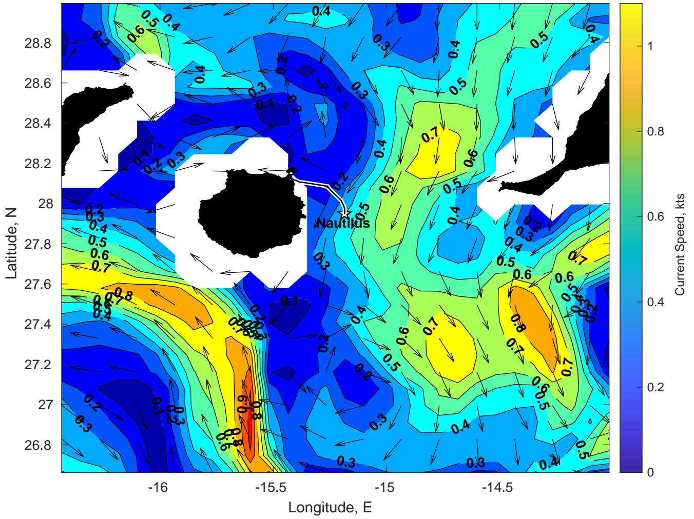
Surface Currents for Nautilus at 27-Dec-2024 00:00:00
