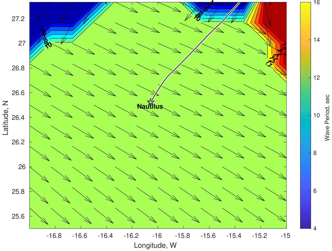
Wave Period (sec) for Nautilus at 28-Dec-2024 09:00:00
