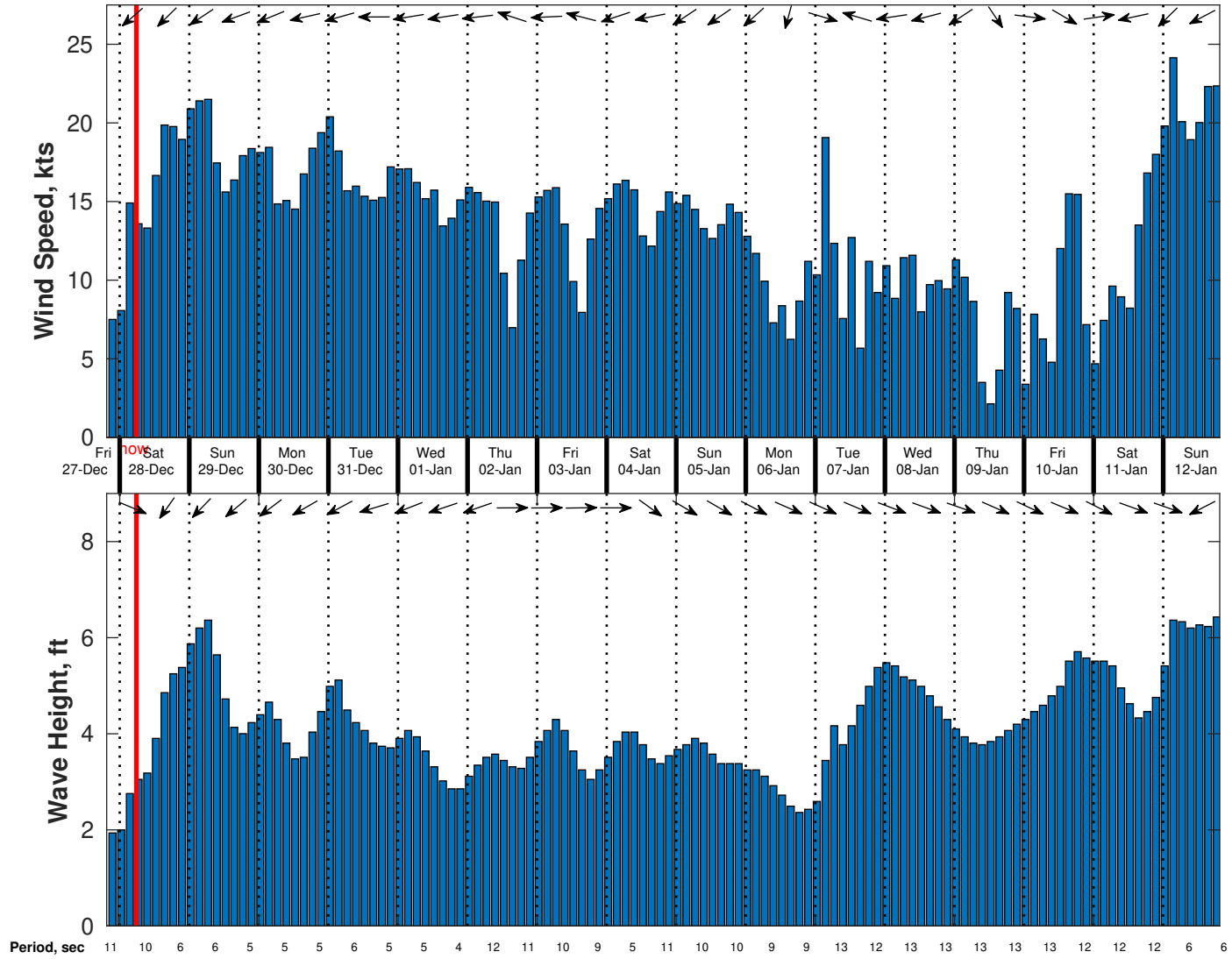
Wind & Wave Forecast for Nautilus from 27-Dec-2024 20:00:00 to 12-Jan-2025 20:00:00
