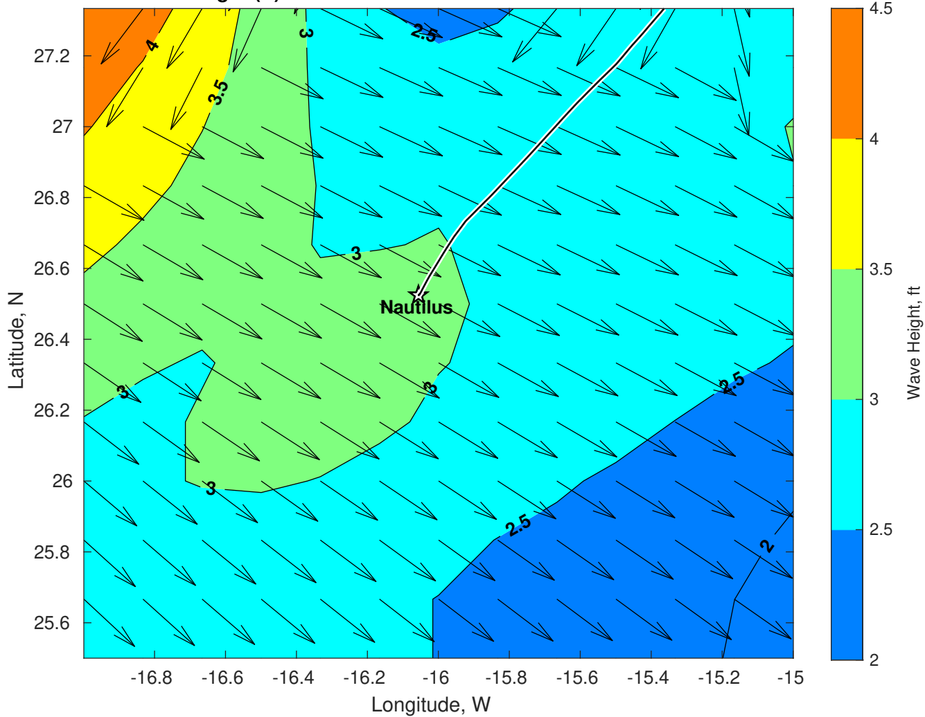
Wave Height (ft) for Nautilus at 28-Dec-2024 09:00:00
