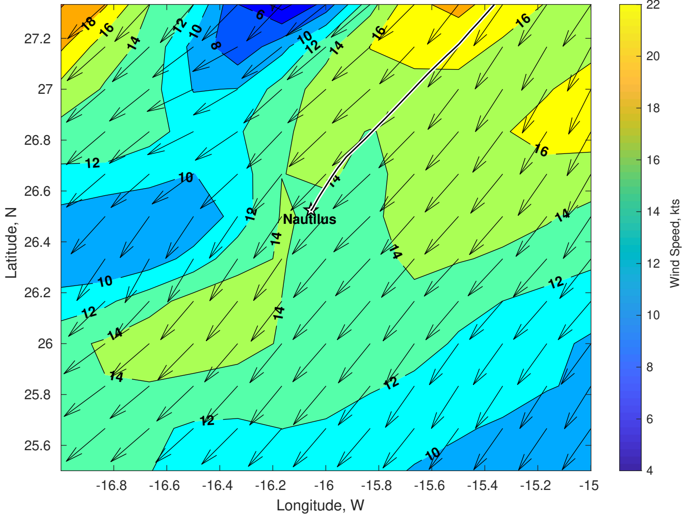
Winds (kts) for Nautilus at 28-Dec-2024 09:00:00
