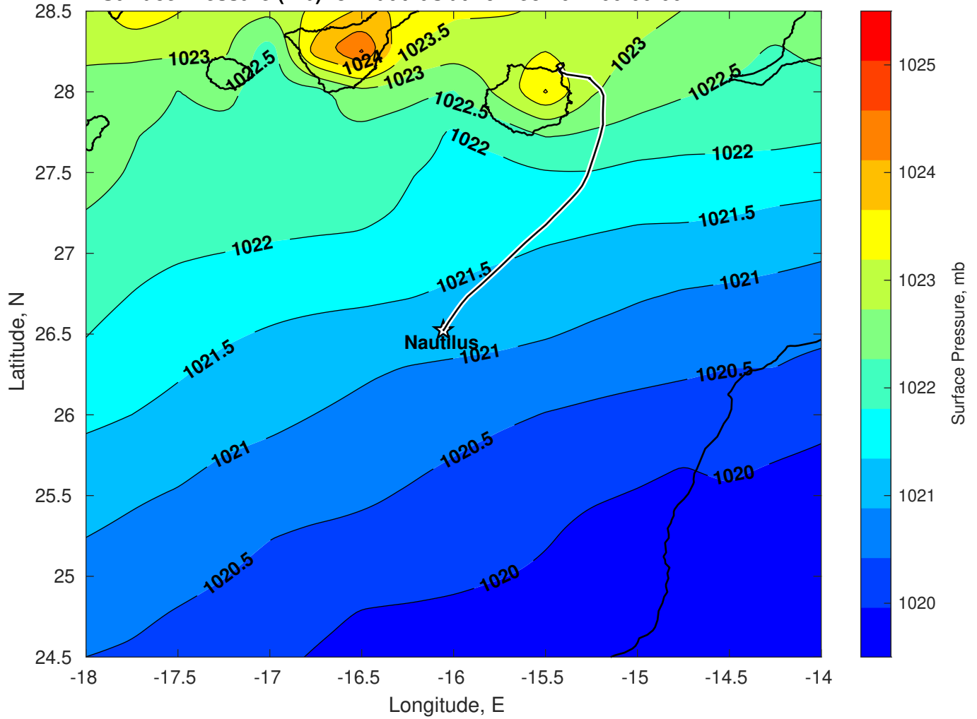
Surface Pressure (mb) for Nautilus at 29-Dec-2024 00:00:00
