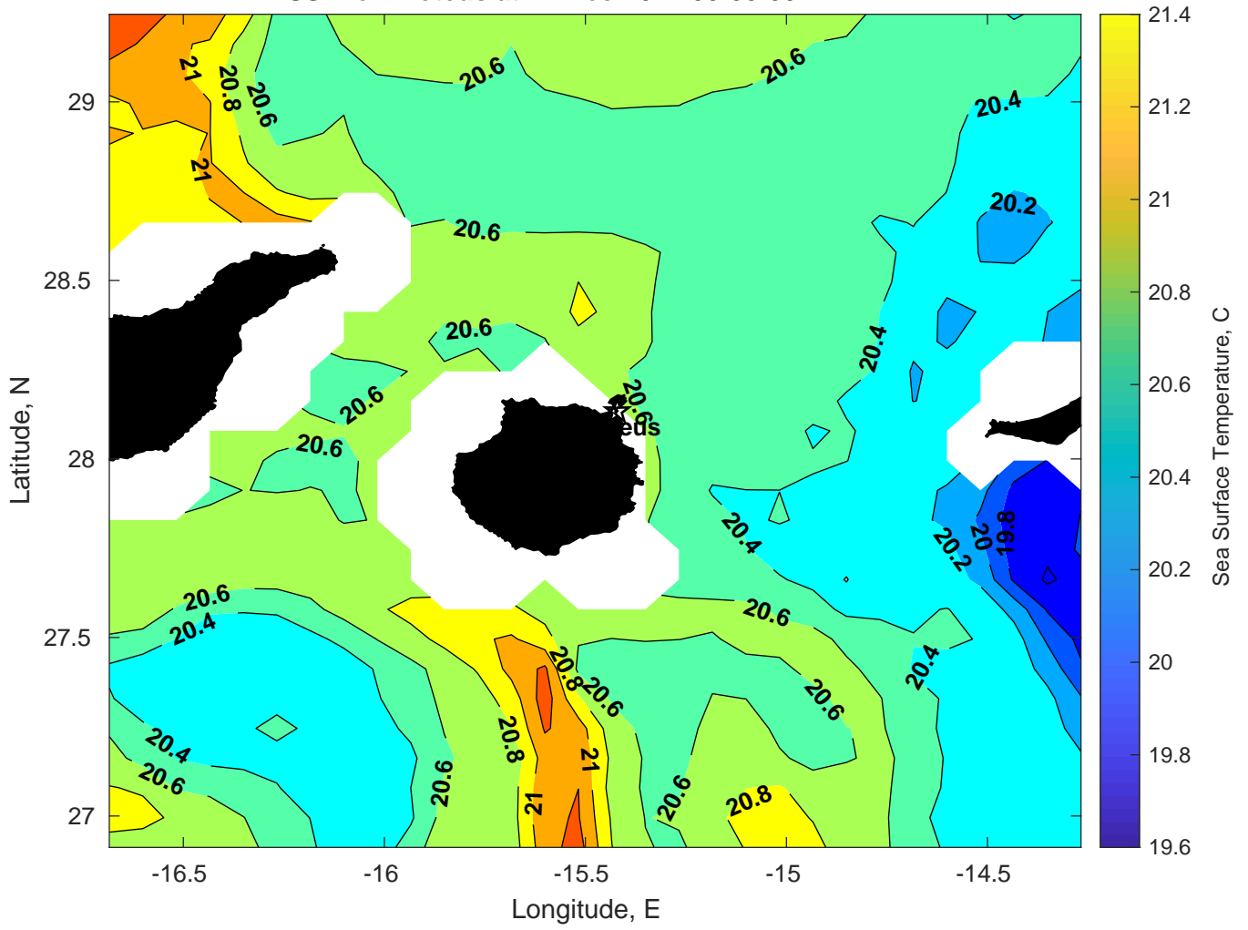
SST for Proteus at 27-Dec-2024 00:00:00
