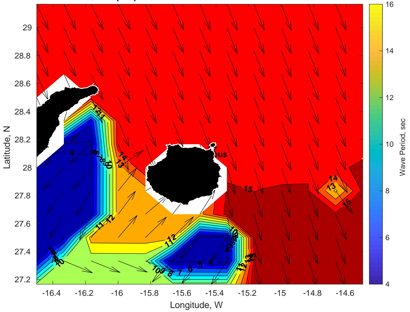
Wave Period (sec) for Proteus at 28-Dec-2024 09:00:00
