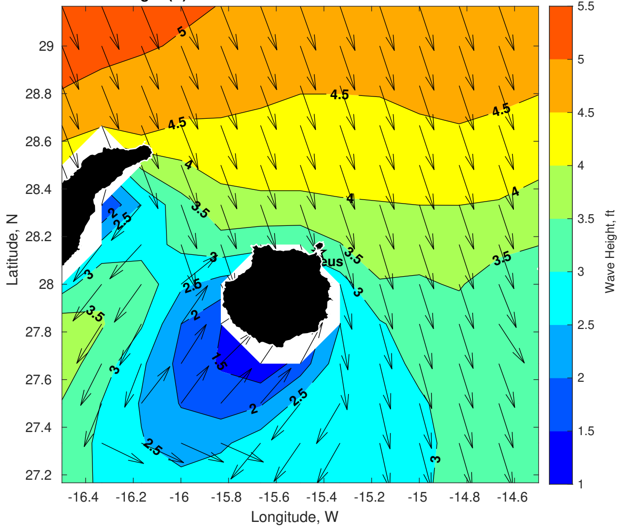
Wave Height (ft) for Proteus at 28-Dec-2024 09:00:00
