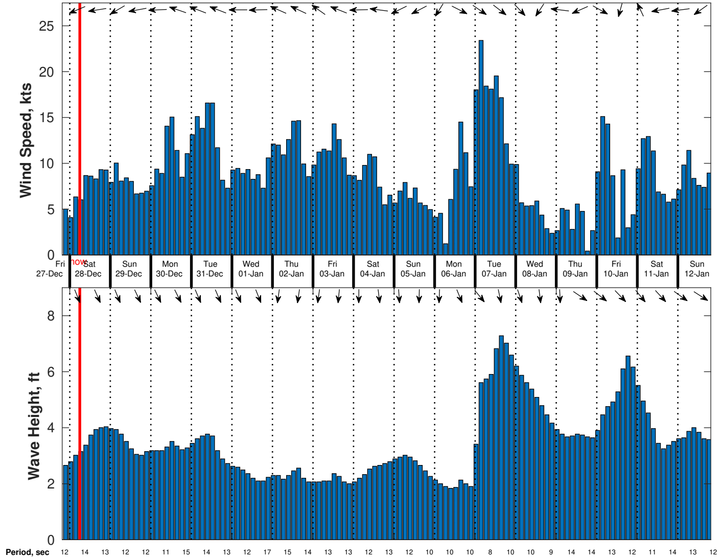
Wind & Wave Forecast for Proteus from 27-Dec-2024 20:00:00 to 12-Jan-2025 20:00:00
