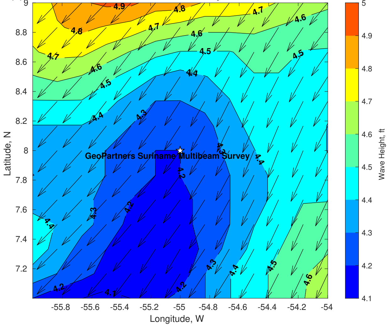
Wave Height (ft) for GeoPartners Suriname Multibeam Survey at 27-Dec-2024 21:00:00
