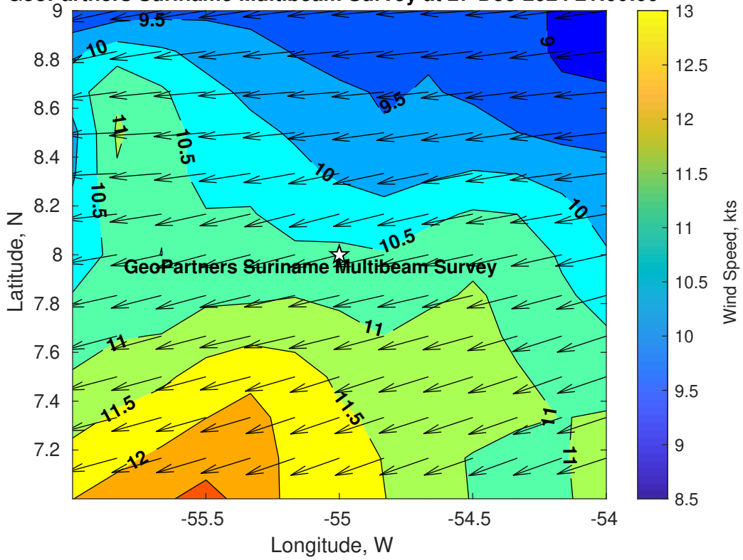
Winds (kts) for GeoPartners Suriname Multibeam Survey at 27-Dec-2024 21:00:00
