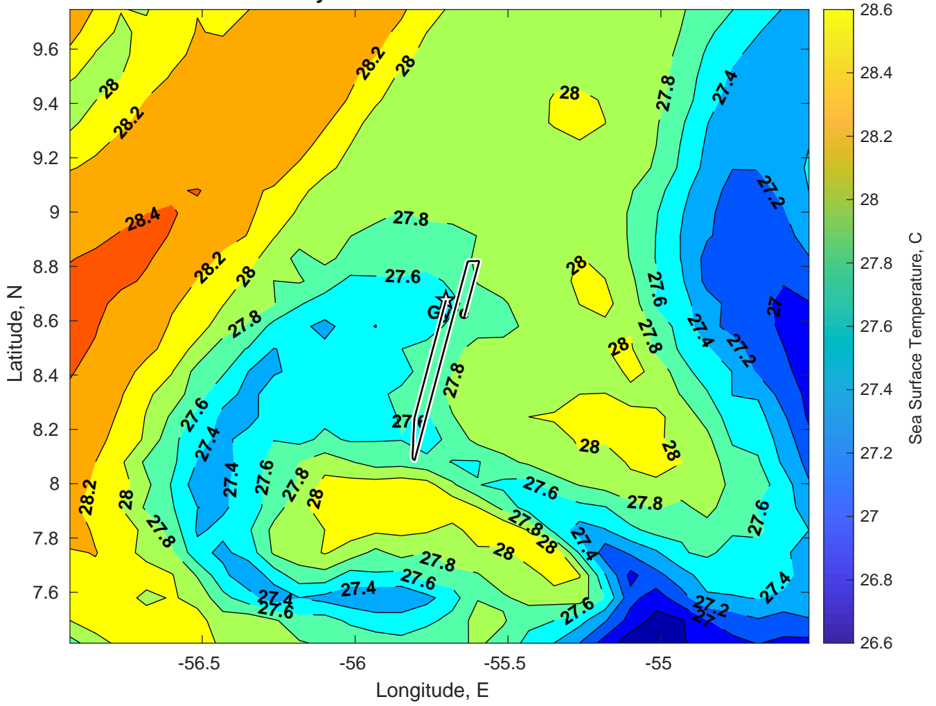
SST for Gyre at 28-Dec-2024 00:00:00
