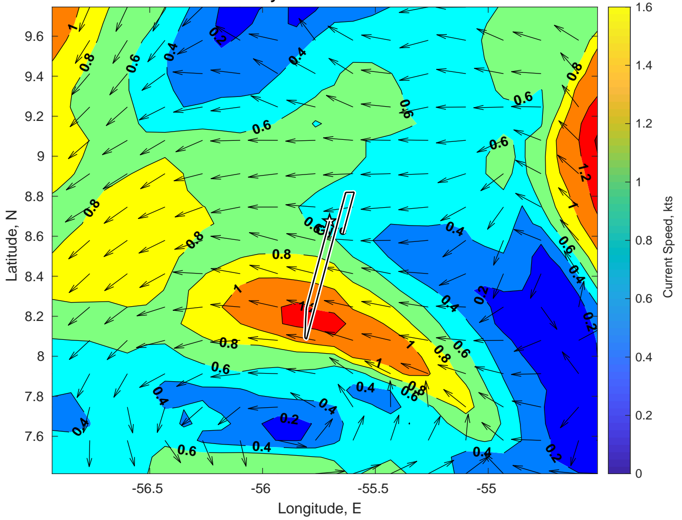
Surface Currents for Gyre at 28-Dec-2024 00:00:00
