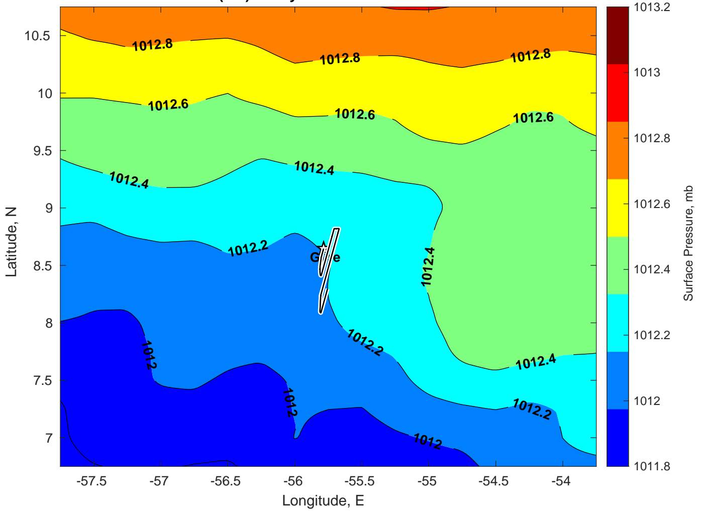
Surface Pressure (mb) for Gyre at 29-Dec-2024 00:00:00
