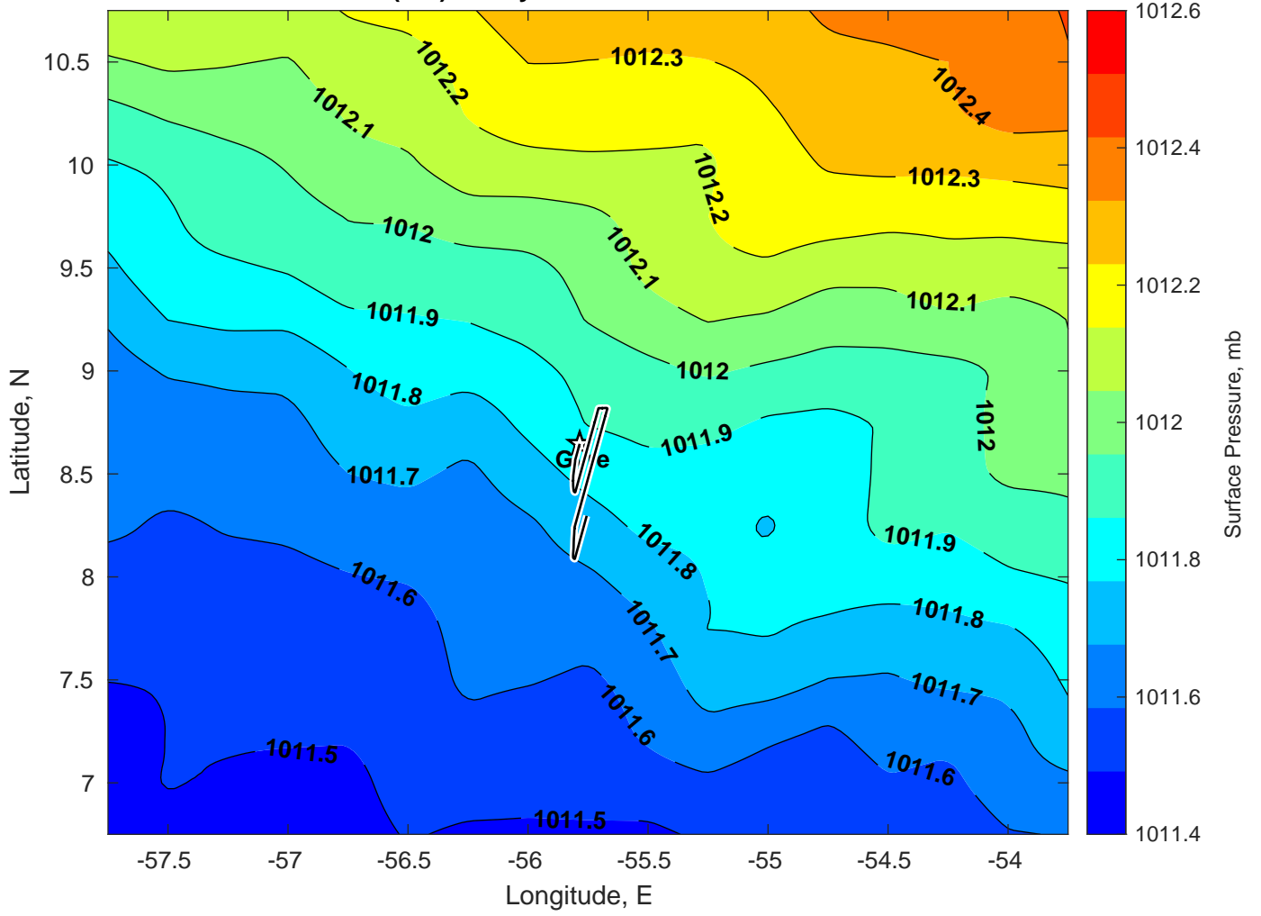
Surface Pressure (mb) for Gyre at 30-Dec-2024 00:00:00
