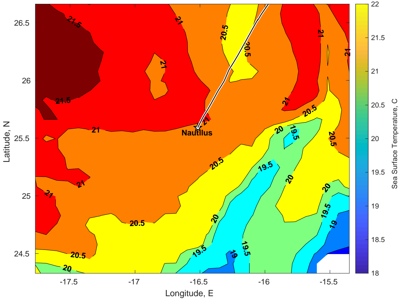
SST for Nautilus at 28-Dec-2024 00:00:00
