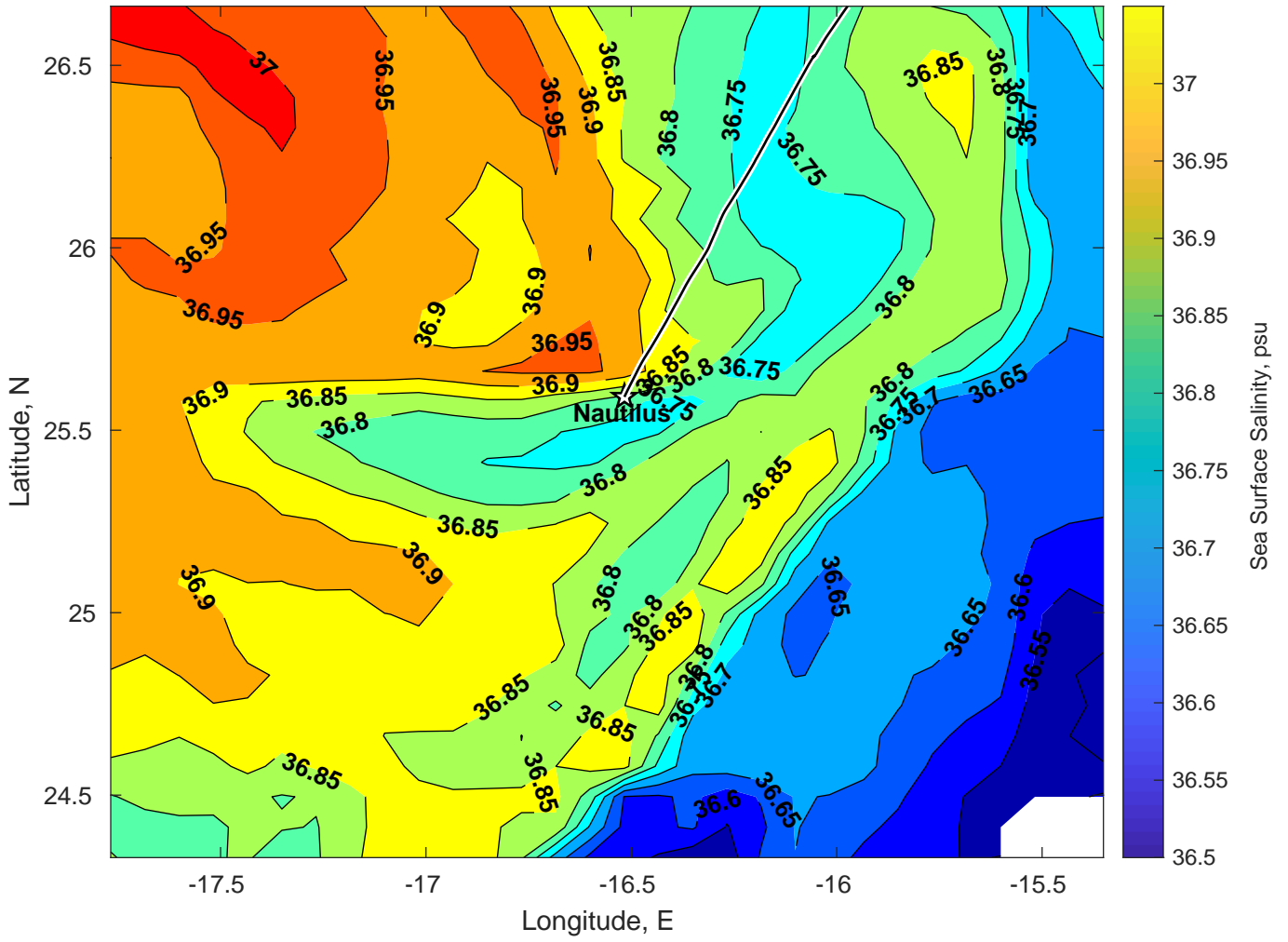
Surface Salinity for Nautilus at 28-Dec-2024 00:00:00
