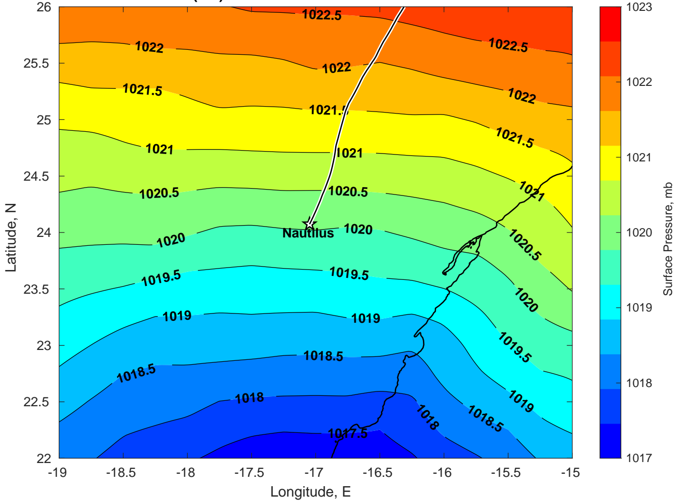
Surface Pressure (mb) for Nautilus at 31-Dec-2024 00:00:00
