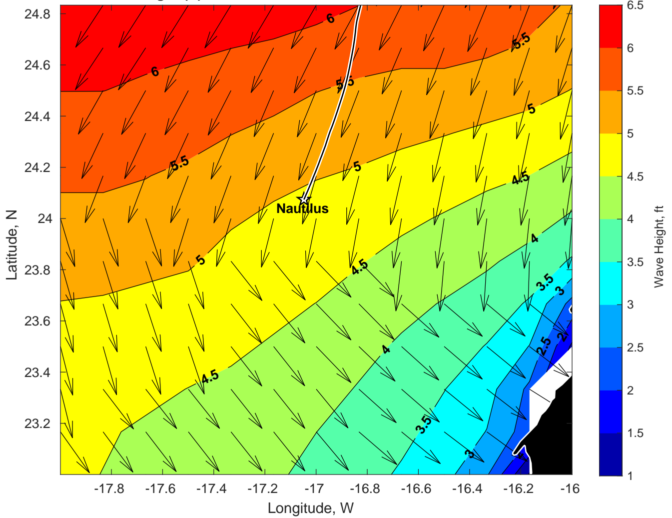
Wave Height (ft) for Nautilus at 29-Dec-2024 09:00:00
