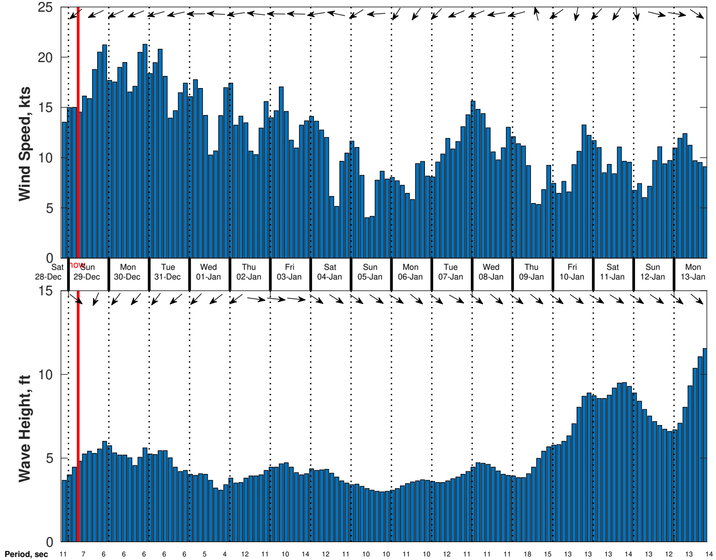
Wind & Wave Forecast for Nautilus from 28-Dec-2024 20:00:00 to 13-Jan-2025 20:00:00
