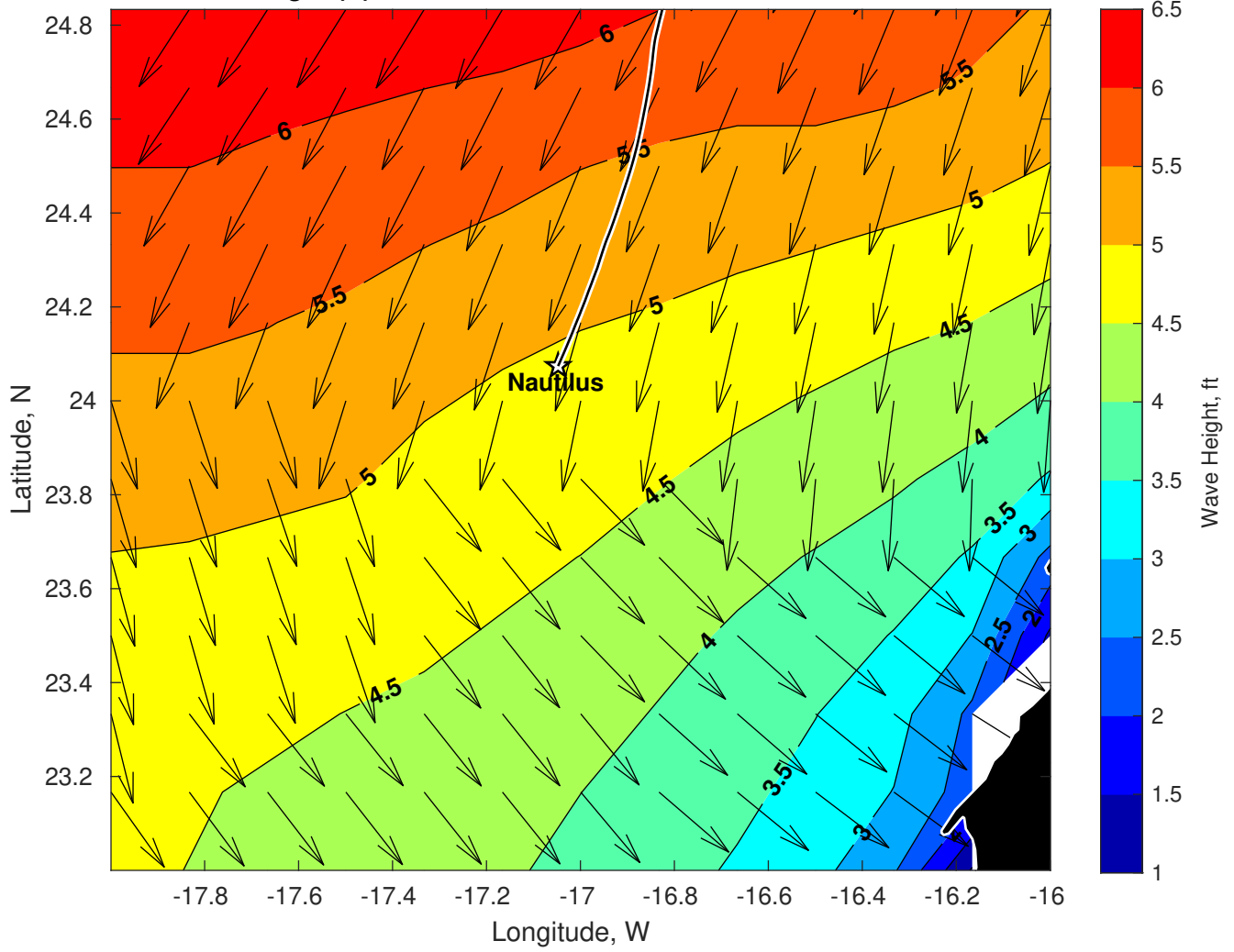
Wave Height (ft) for Nautilus at 29-Dec-2024 09:00:00
