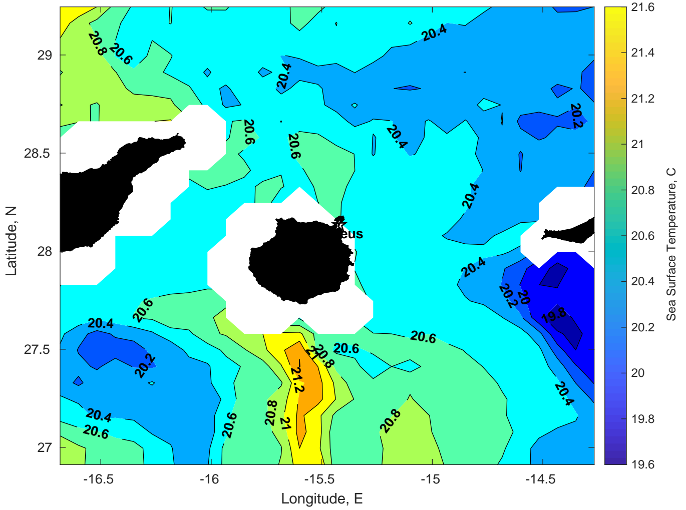
SST for Proteus at 28-Dec-2024 00:00:00
