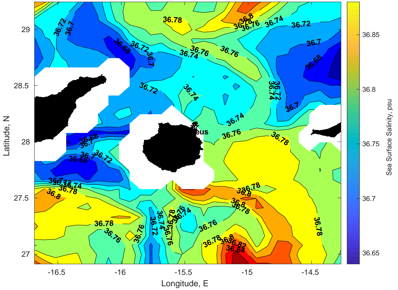
Surface Salinity for Proteus at 28-Dec-2024 00:00:00
