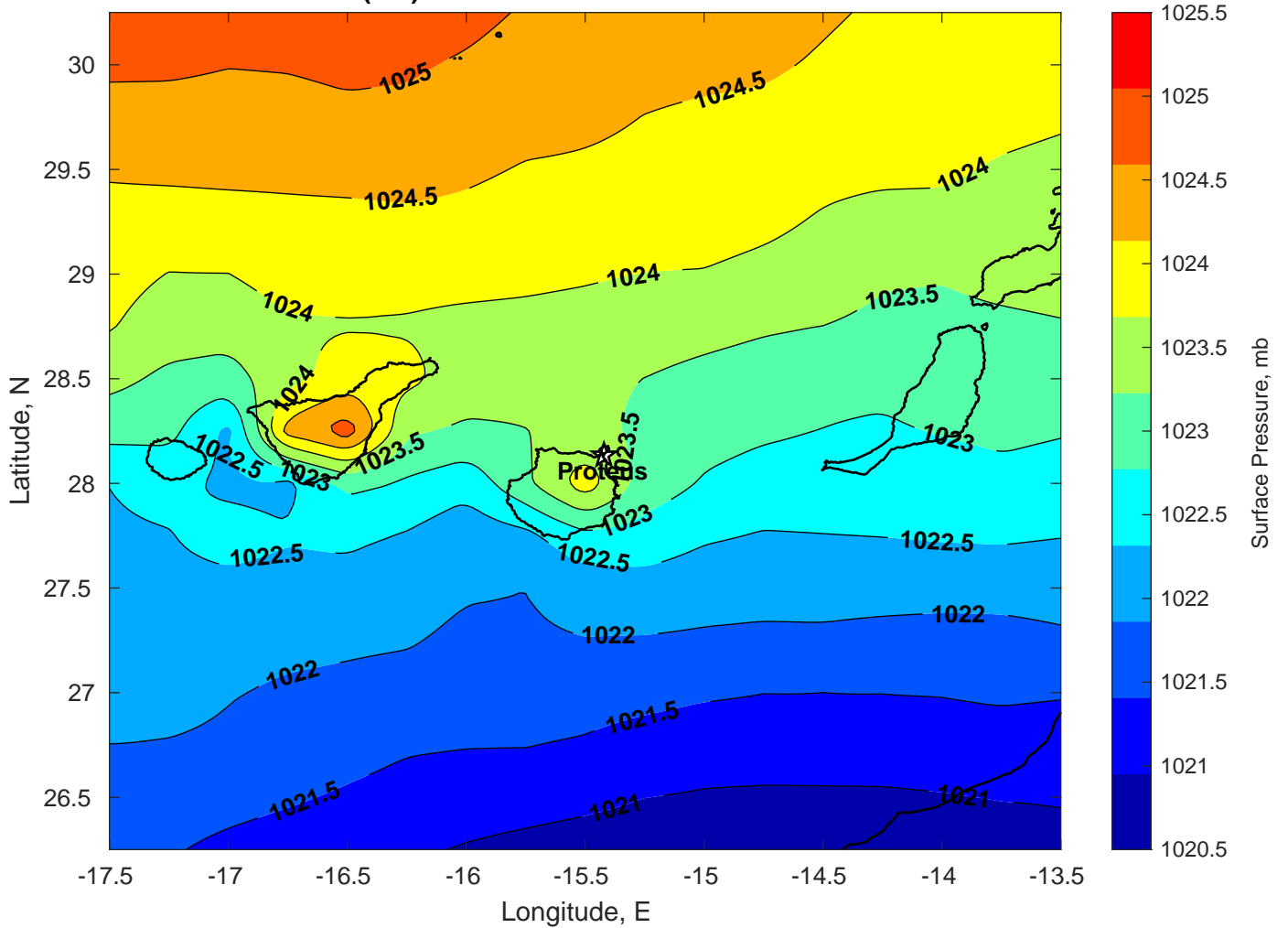
Surface Pressure (mb) for Proteus at 29-Dec-2024 00:00:00
