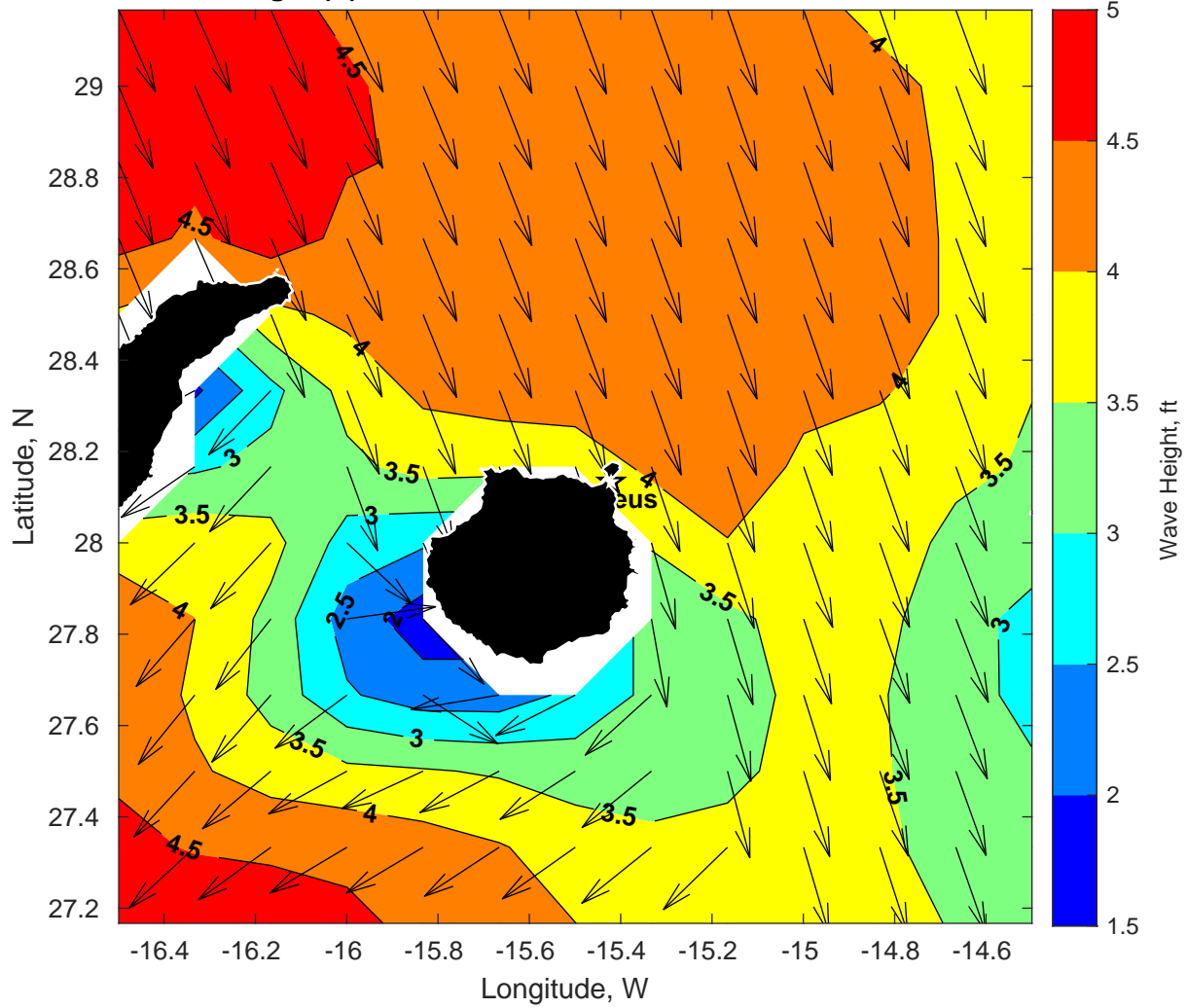
Wave Height (ft) for Proteus at 29-Dec-2024 09:00:00
