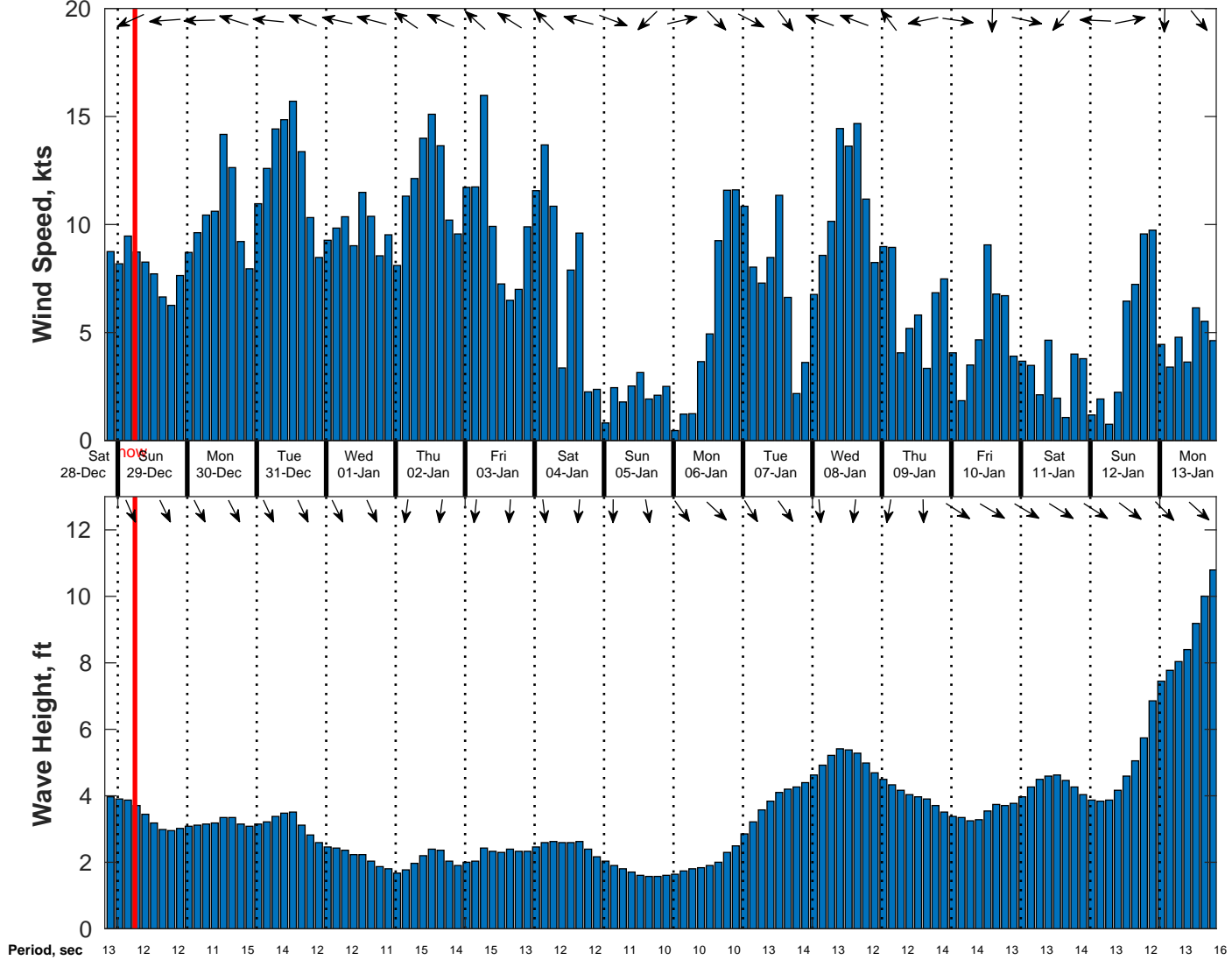
Wind & Wave Forecast for Proteus from 28-Dec-2024 20:00:00 to 13-Jan-2025 20:00:00
