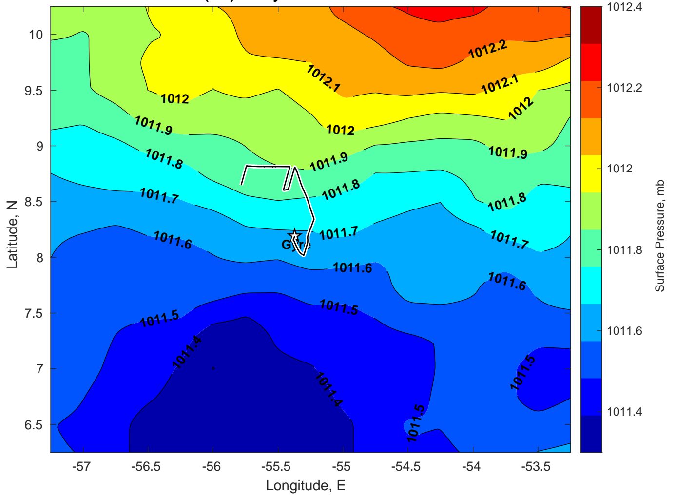
Surface Pressure (mb) for Gyre at 30-Dec-2024 00:00:00
