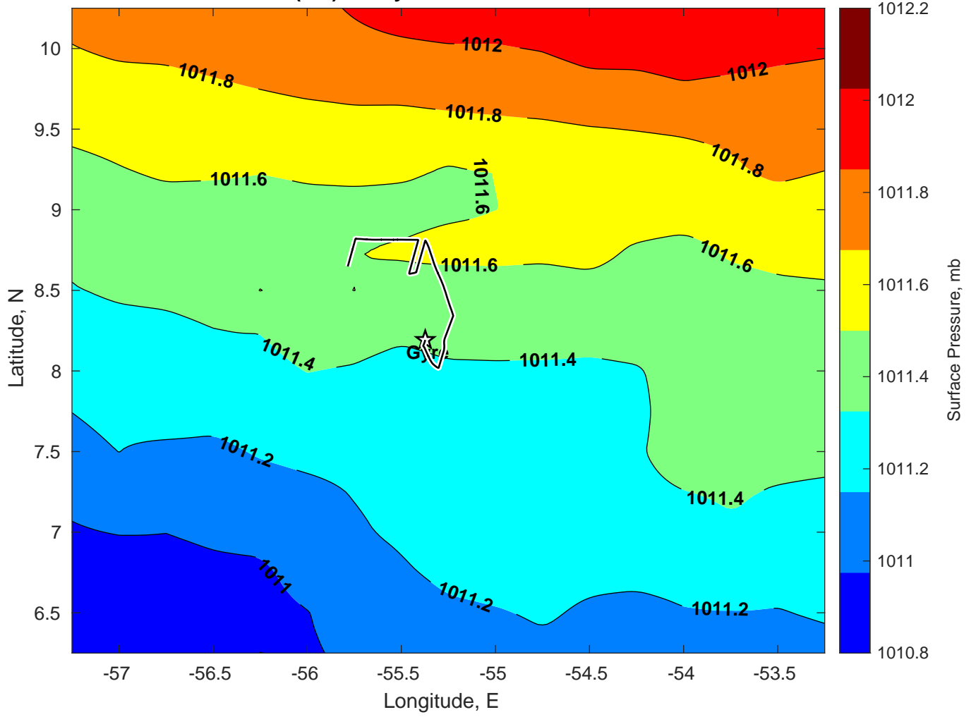
Surface Pressure (mb) for Gyre at 31-Dec-2024 00:00:00
