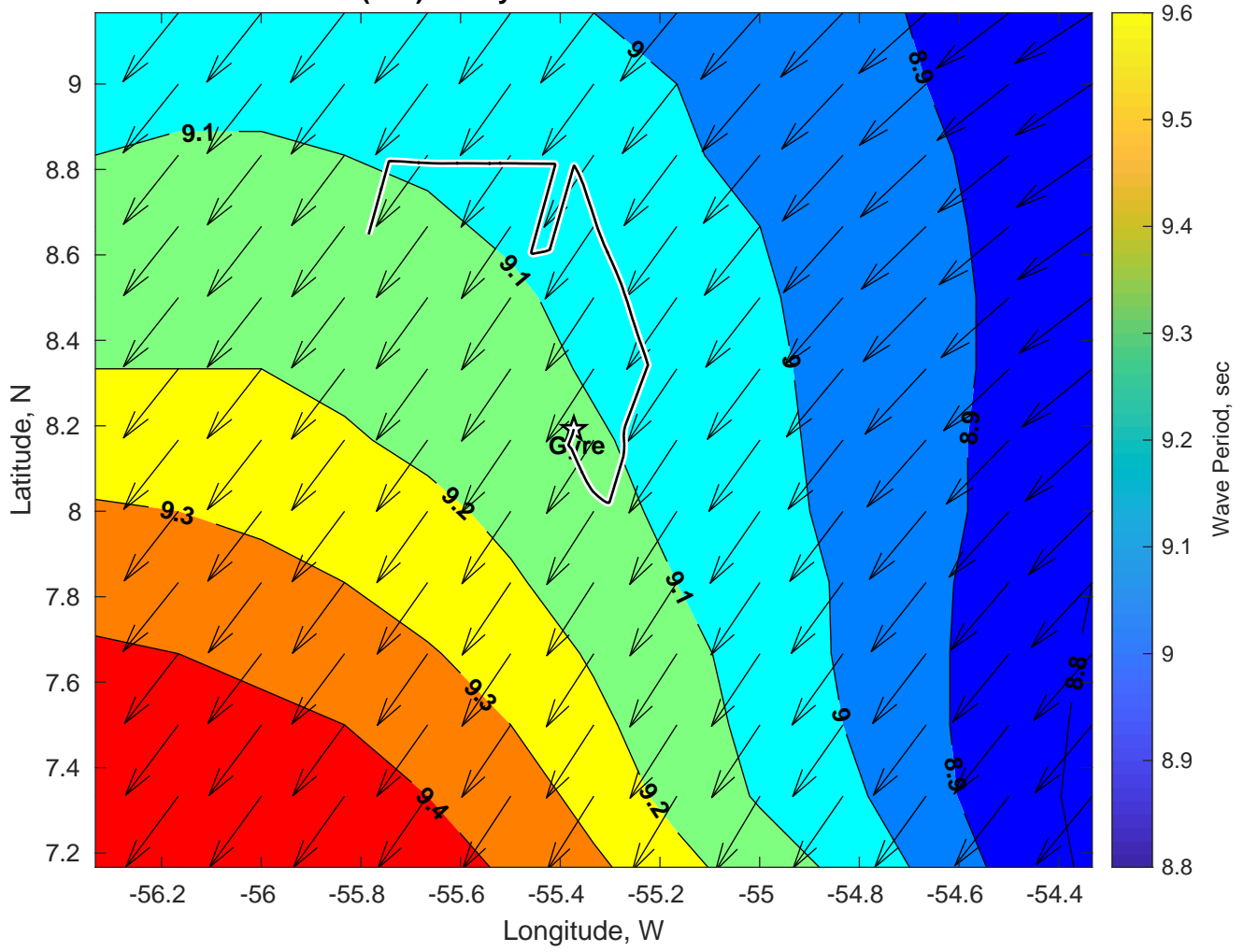
Wave Period (sec) for Gyre at 30-Dec-2024 09:00:00
