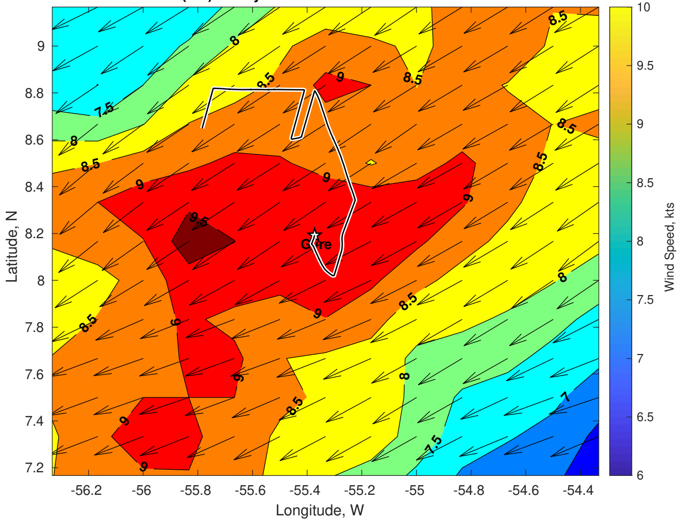
Winds (kts) for Gyre at 30-Dec-2024 09:00:00
