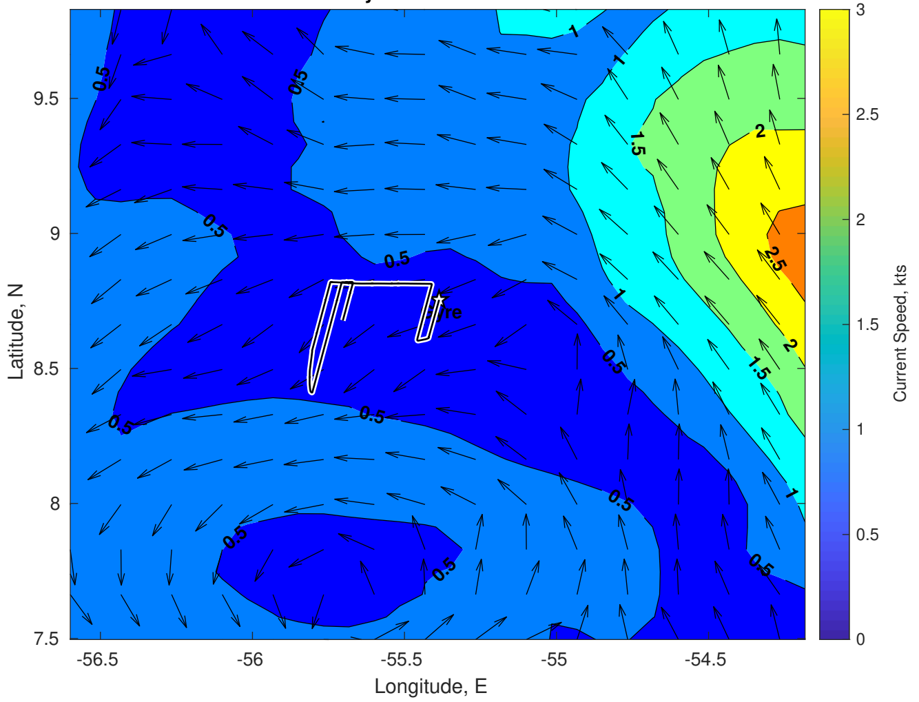
Surface Currents for Gyre at 29-Dec-2024 00:00:00
