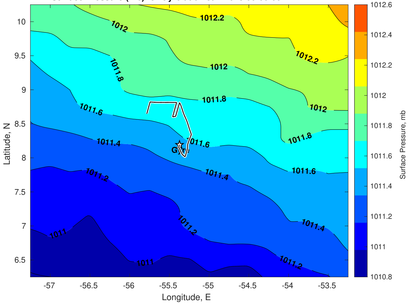
Surface Pressure (mb) for Gyre at 01-Jan-2025 00:00:00
