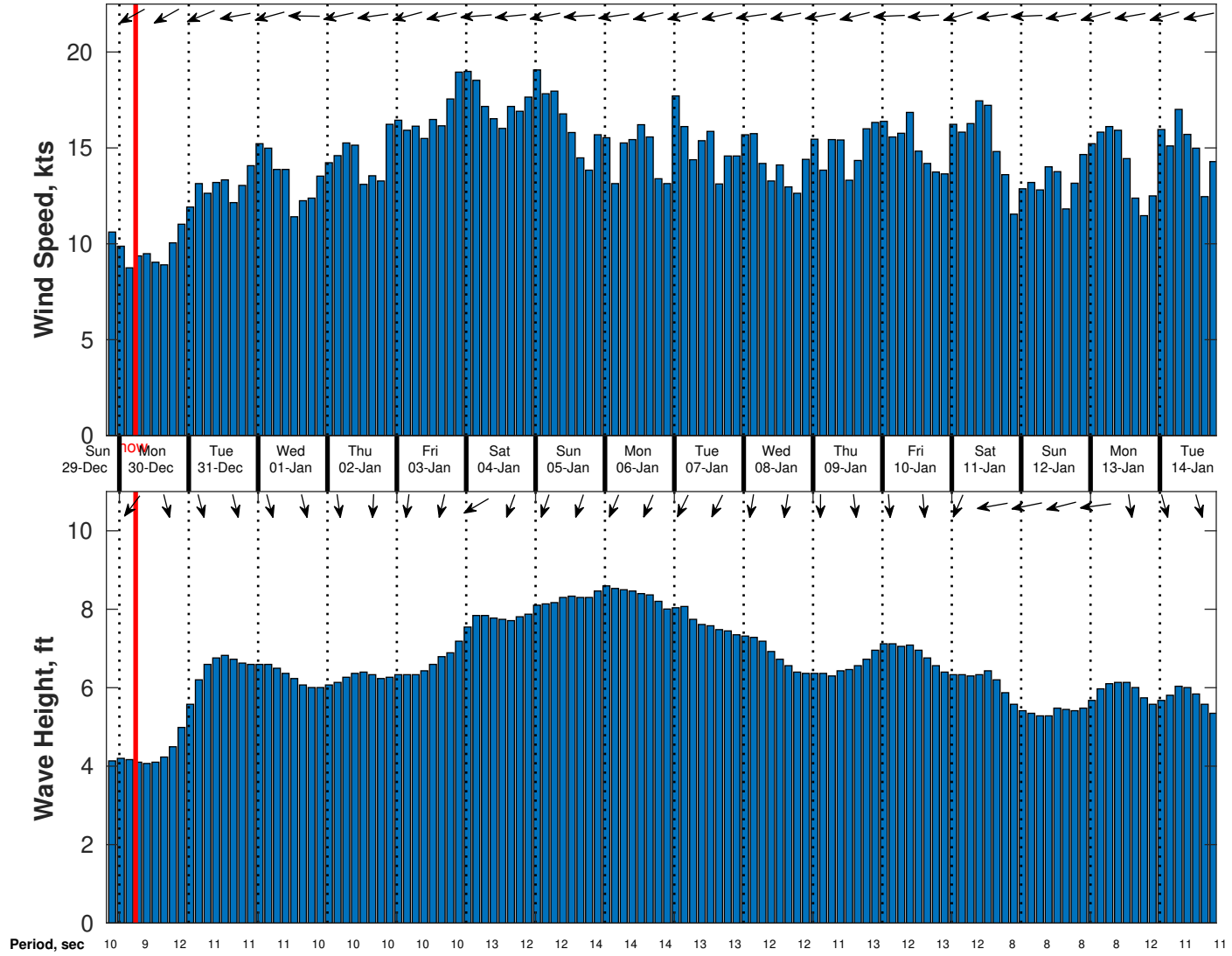
Wind & Wave Forecast for Gyre from 29-Dec-2024 20:00:00 to 14-Jan-2025 20:00:00
