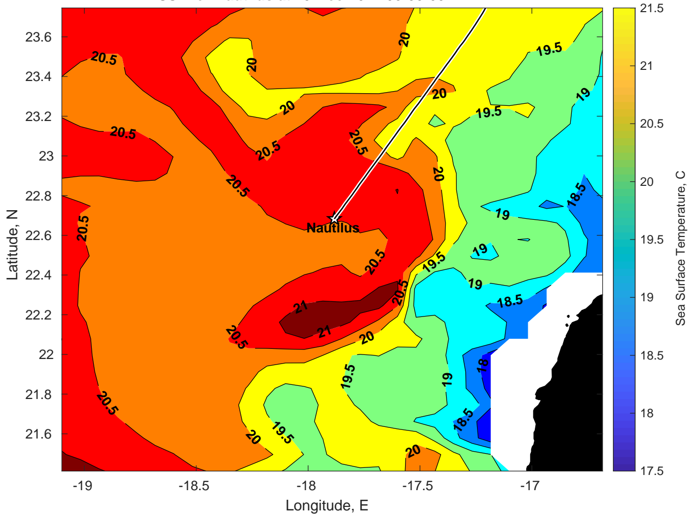
SST for Nautilus at 29-Dec-2024 00:00:00
