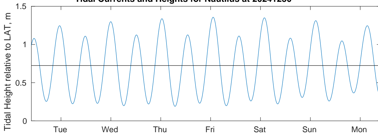
Tidal Currents and Heights for Nautilus at 20241230
