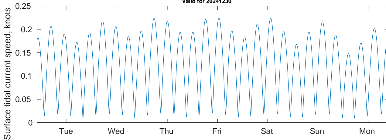
Tidal Currents and Heights for Nautilus at 20241230
