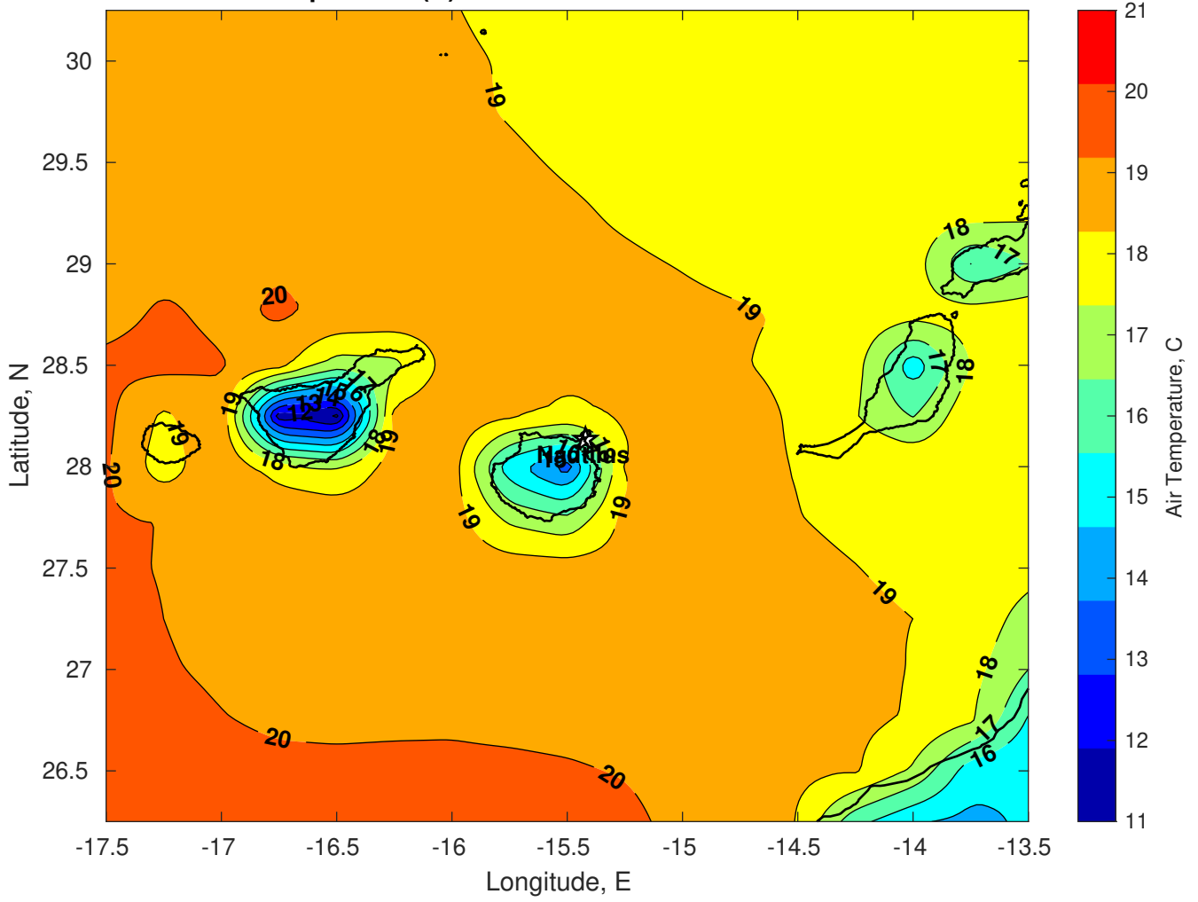
Air Temperature (C) for Nautilus at 31-Dec-2024
