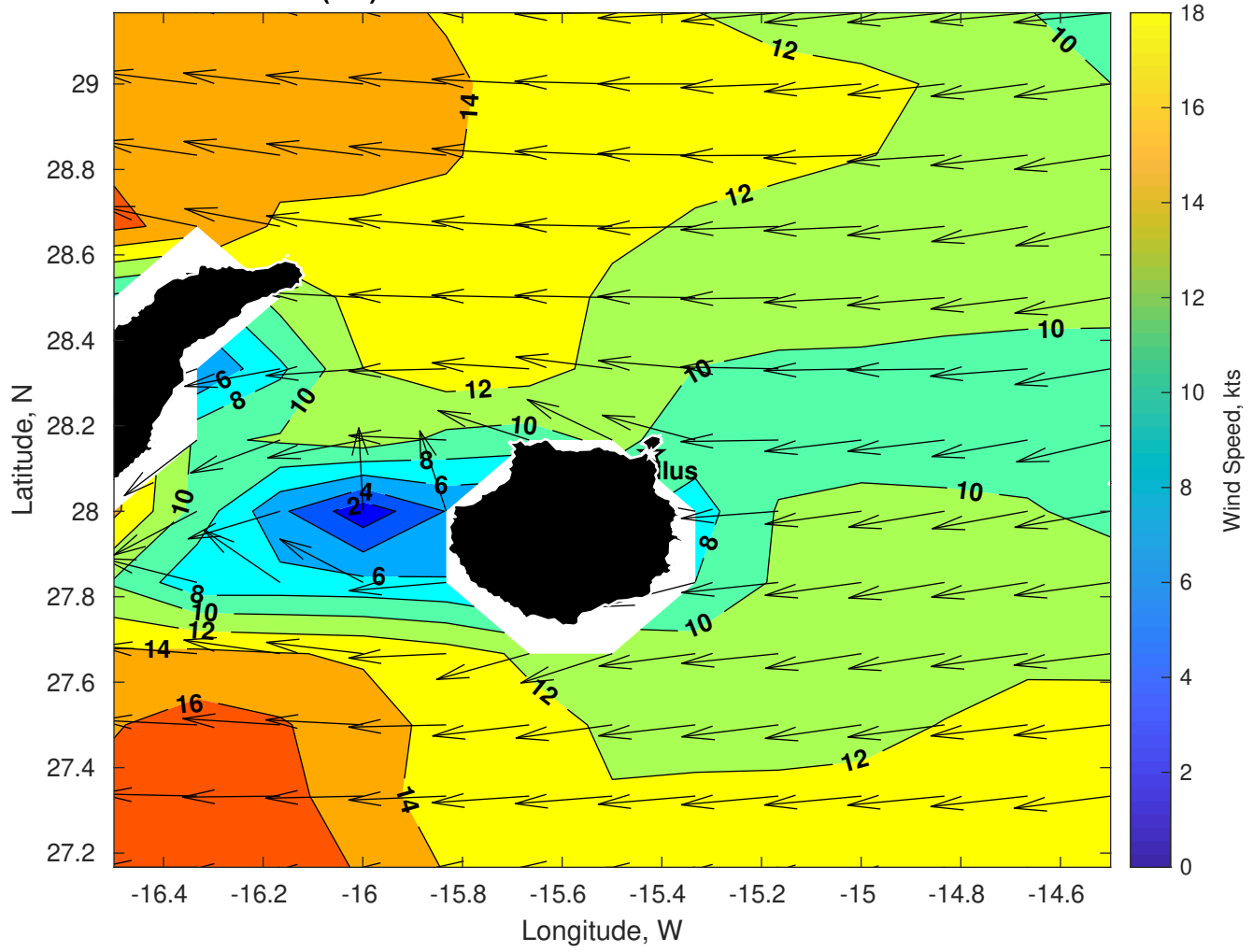
Winds (kts) for Nautilus at 31-Dec-2024 09:00:00
