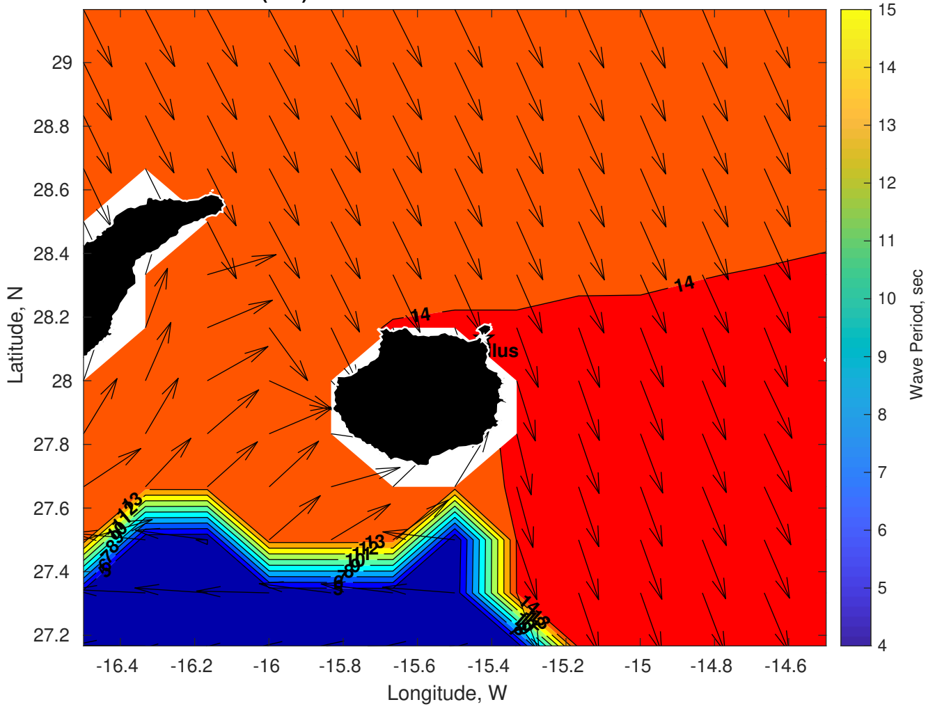
Wave Period (sec) for Nautilus at 31-Dec-2024 09:00:00
