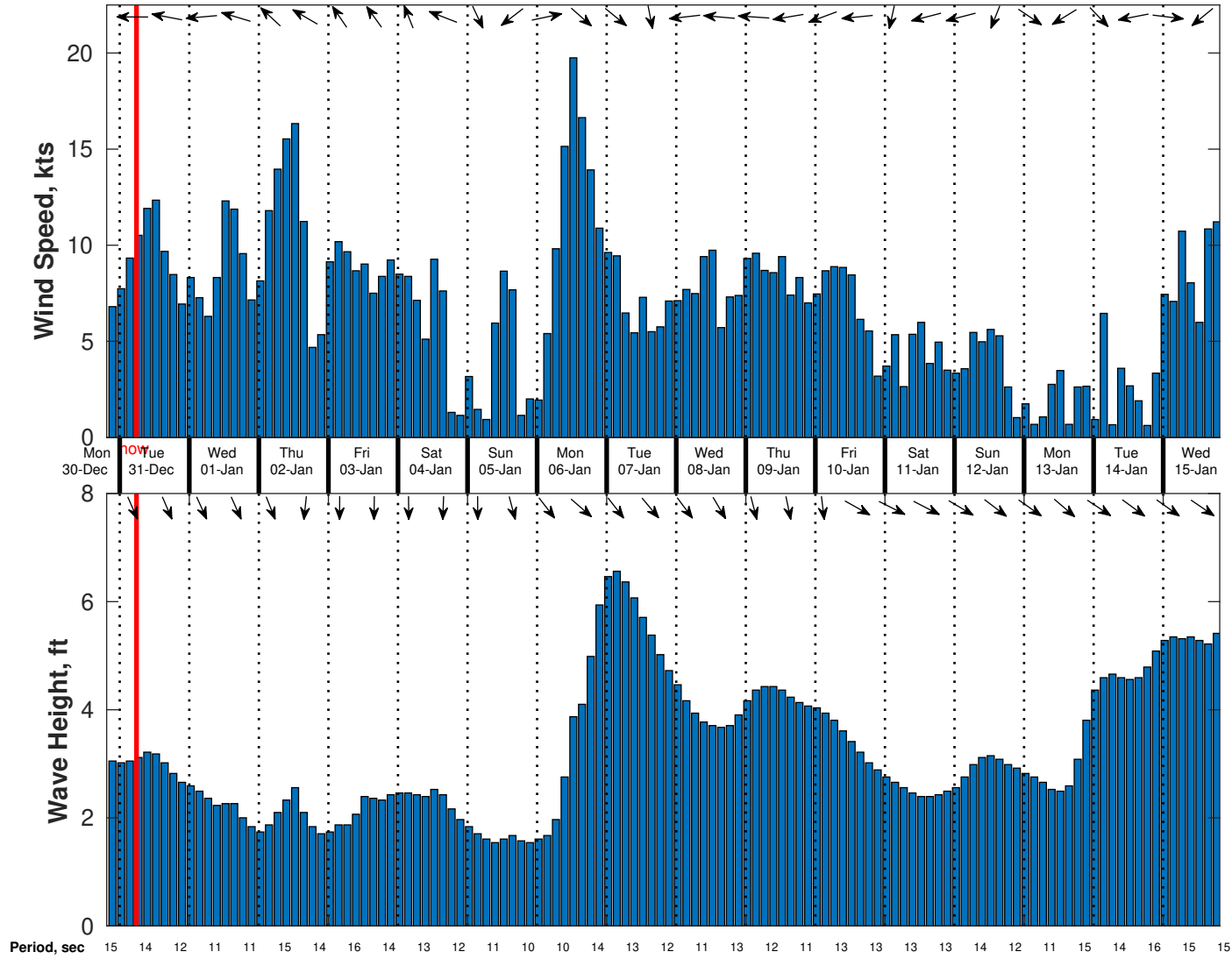
Wind & Wave Forecast for Nautilus from 30-Dec-2024 20:00:00 to 15-Jan-2025 20:00:00
