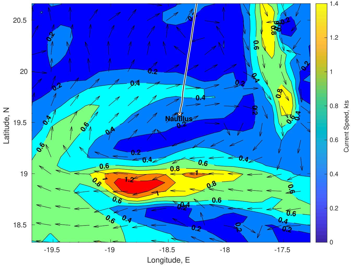
Surface Currents for Nautilus at 30-Dec-2024 00:00:00
