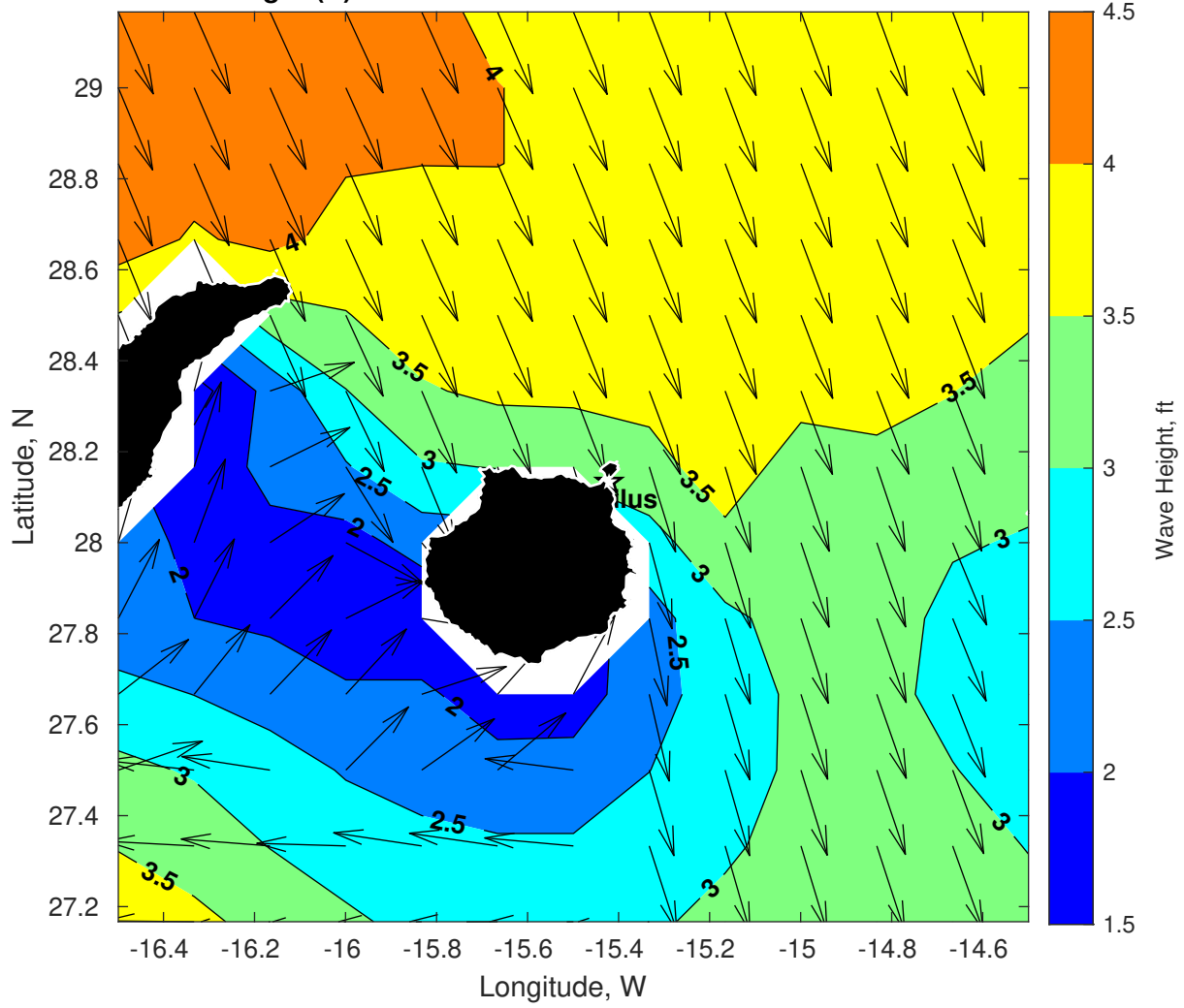
Wave Height (ft) for Nautilus at 31-Dec-2024 09:00:00
