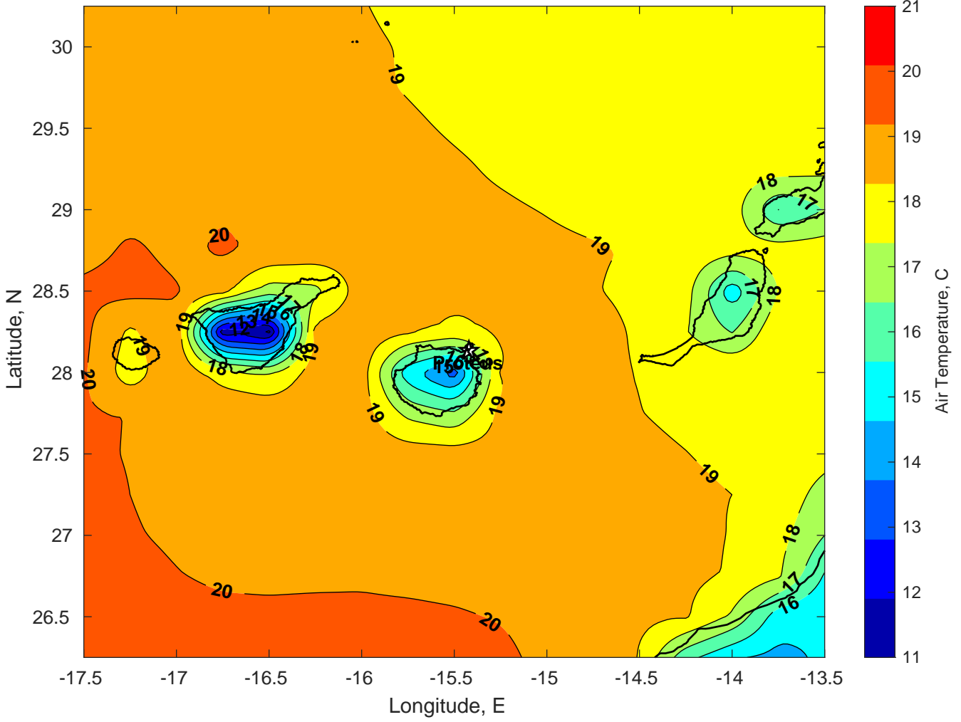
Air Temperature (C) for Proteus at 31-Dec-2024
