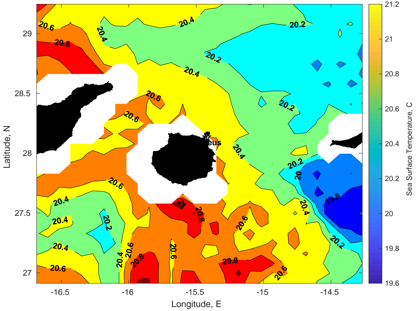
SST for Proteus at 30-Dec-2024 00:00:00
