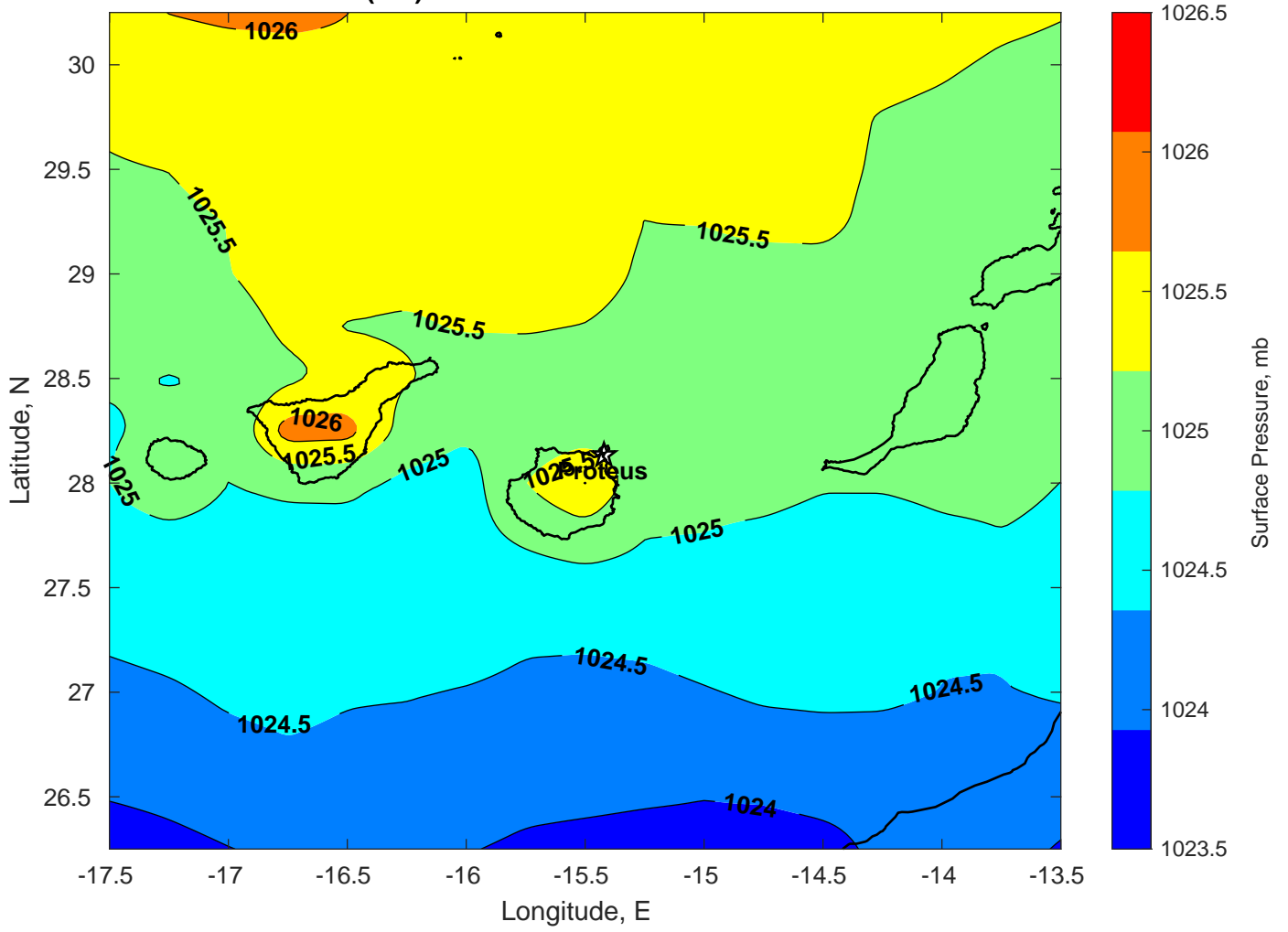
Surface Pressure (mb) for Proteus at 01-Jan-2025 00:00:00
