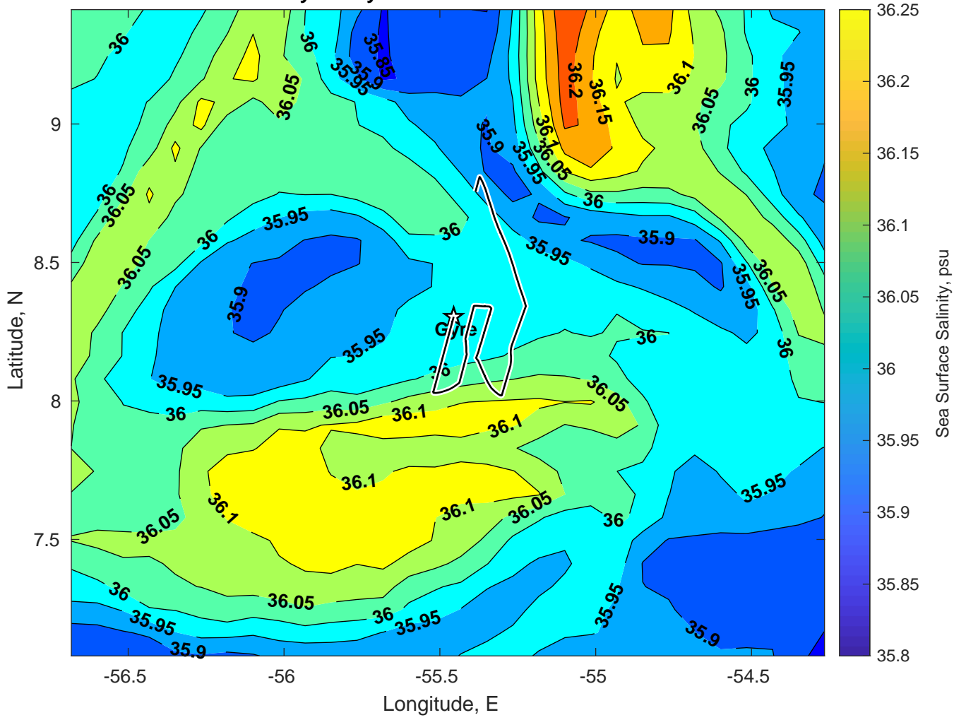
Surface Salinity for Gyre at 30-Dec-2024 00:00:00
