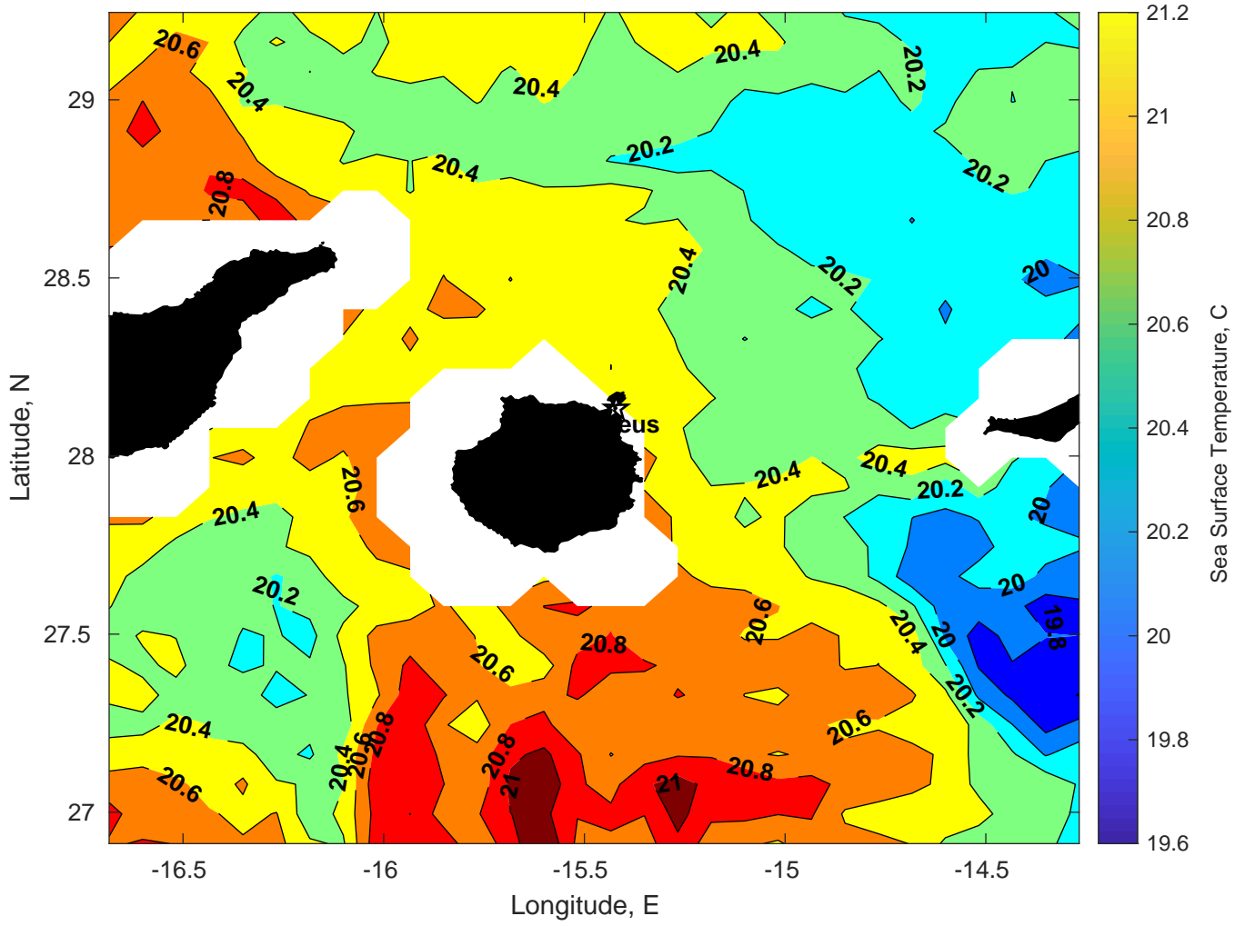
SST for Proteus at 31-Dec-2024 00:00:00
