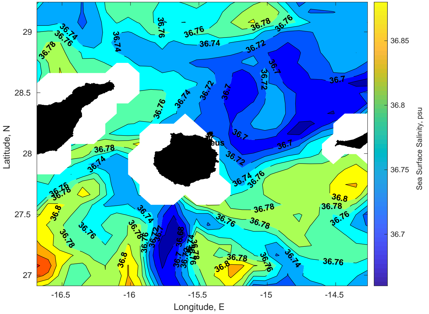
Surface Salinity for Proteus at 31-Dec-2024 00:00:00
