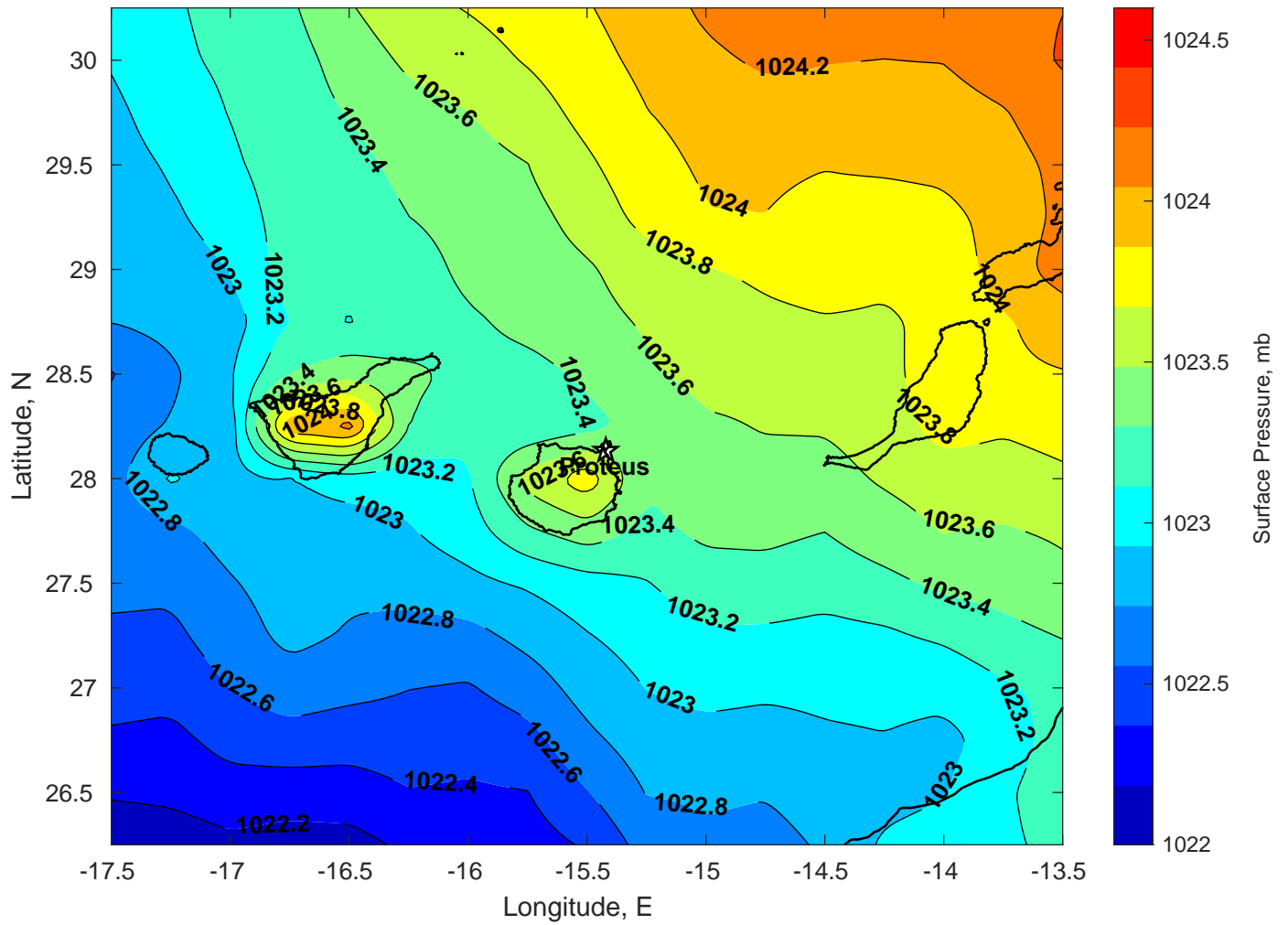
Surface Pressure (mb) for Proteus at 03-Jan-2025 00:00:00
