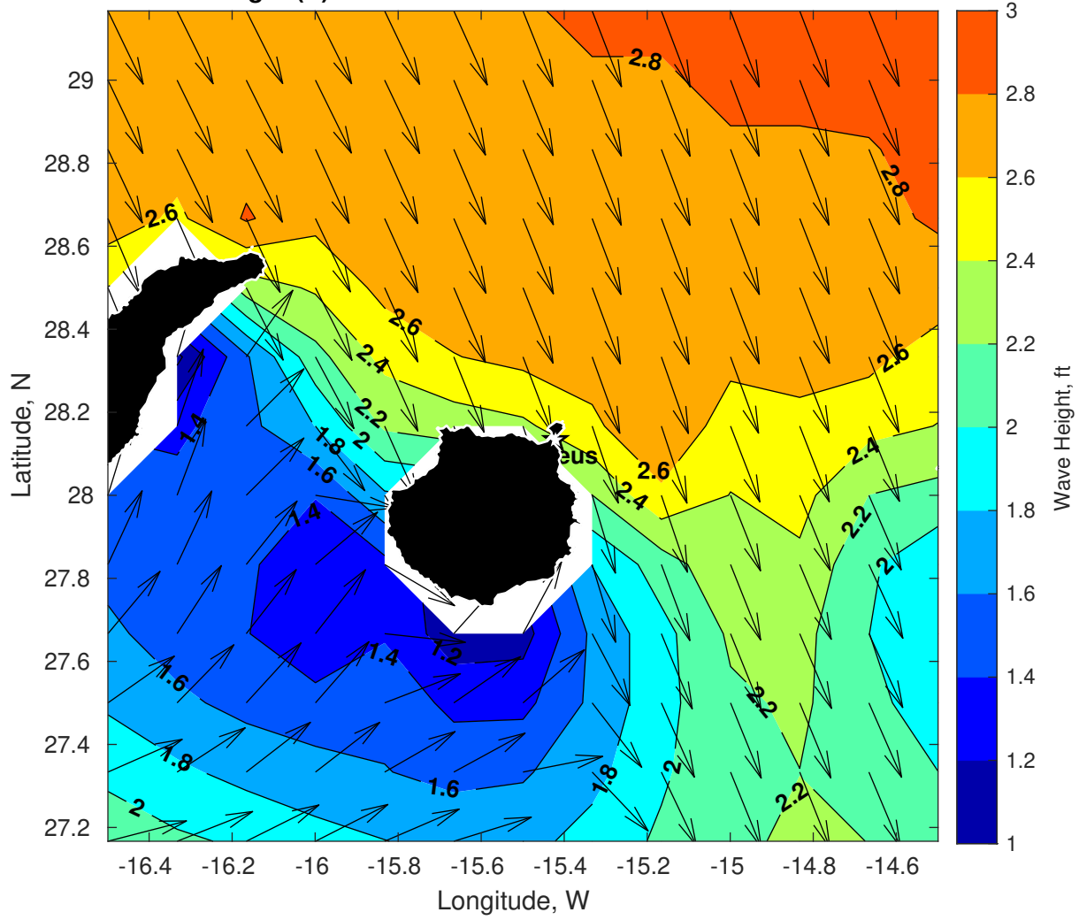
Wave Height (ft) for Proteus at 01-Jan-2025 09:00:00
