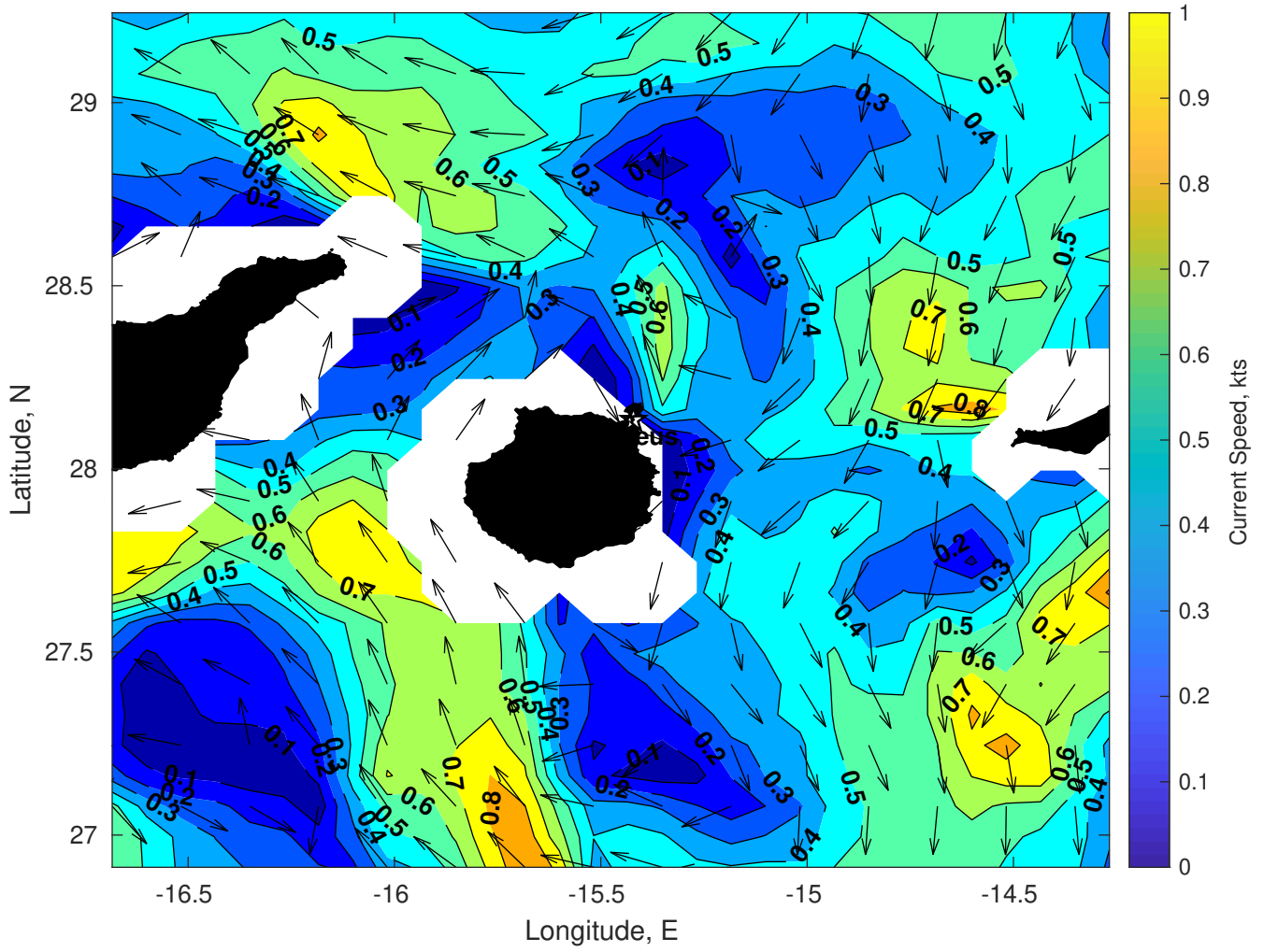
Surface Currents for Proteus at 31-Dec-2024 00:00:00
