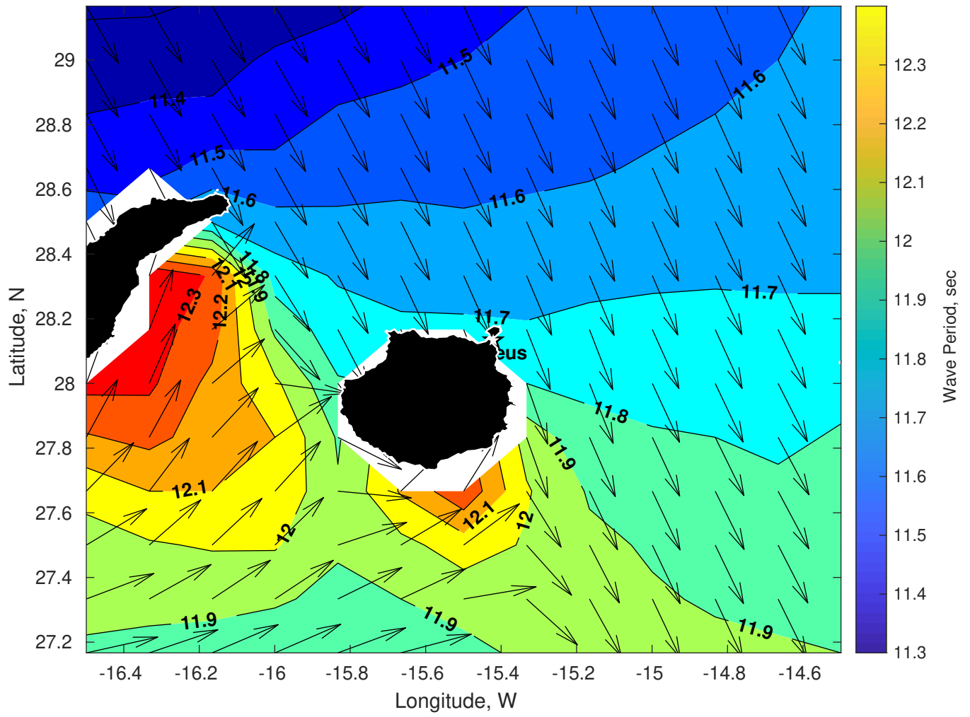
Wave Period (sec) for Proteus at 01-Jan-2025 09:00:00
