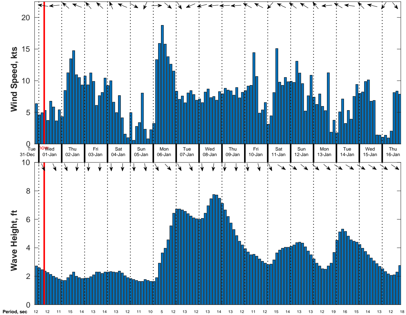
Wind & Wave Forecast for Proteus from 31-Dec-2024 20:00:00 to 16-Jan-2025 20:00:00
