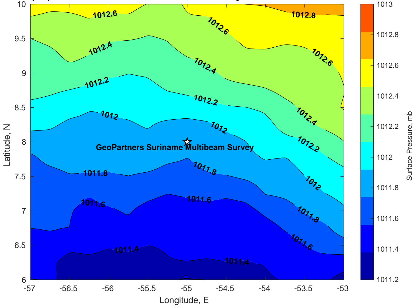
Surface Pressure (mb) for GeoPartners Suriname Multibeam Survey at 04-Jan-2025 00:00:00
