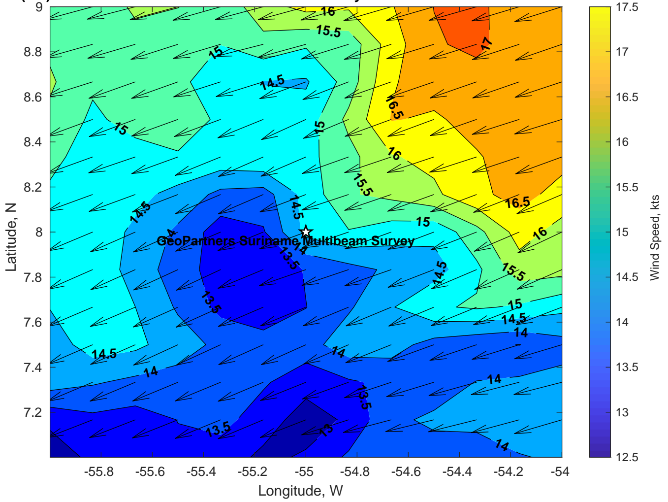
Winds (kts) for GeoPartners Suriname Multibeam Survey at 02-Jan-2025 09:00:00
