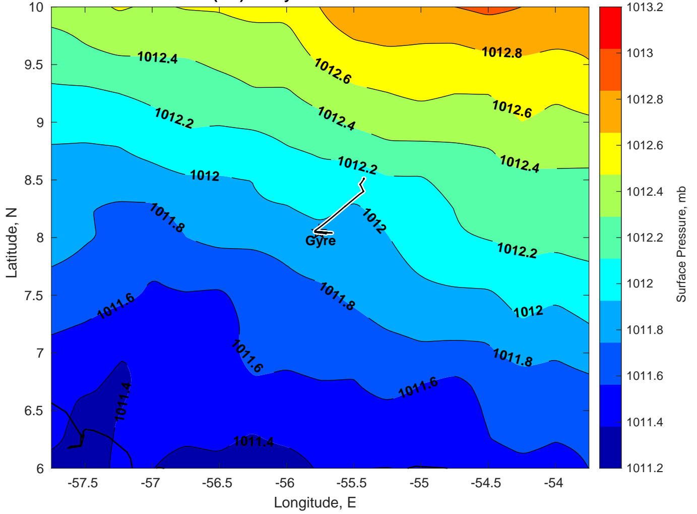
Surface Pressure (mb) for Gyre at 03-Jan-2025 00:00:00
