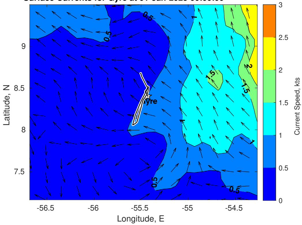
Surface Currents for Gyre at 01-Jan-2025 00:00:00
