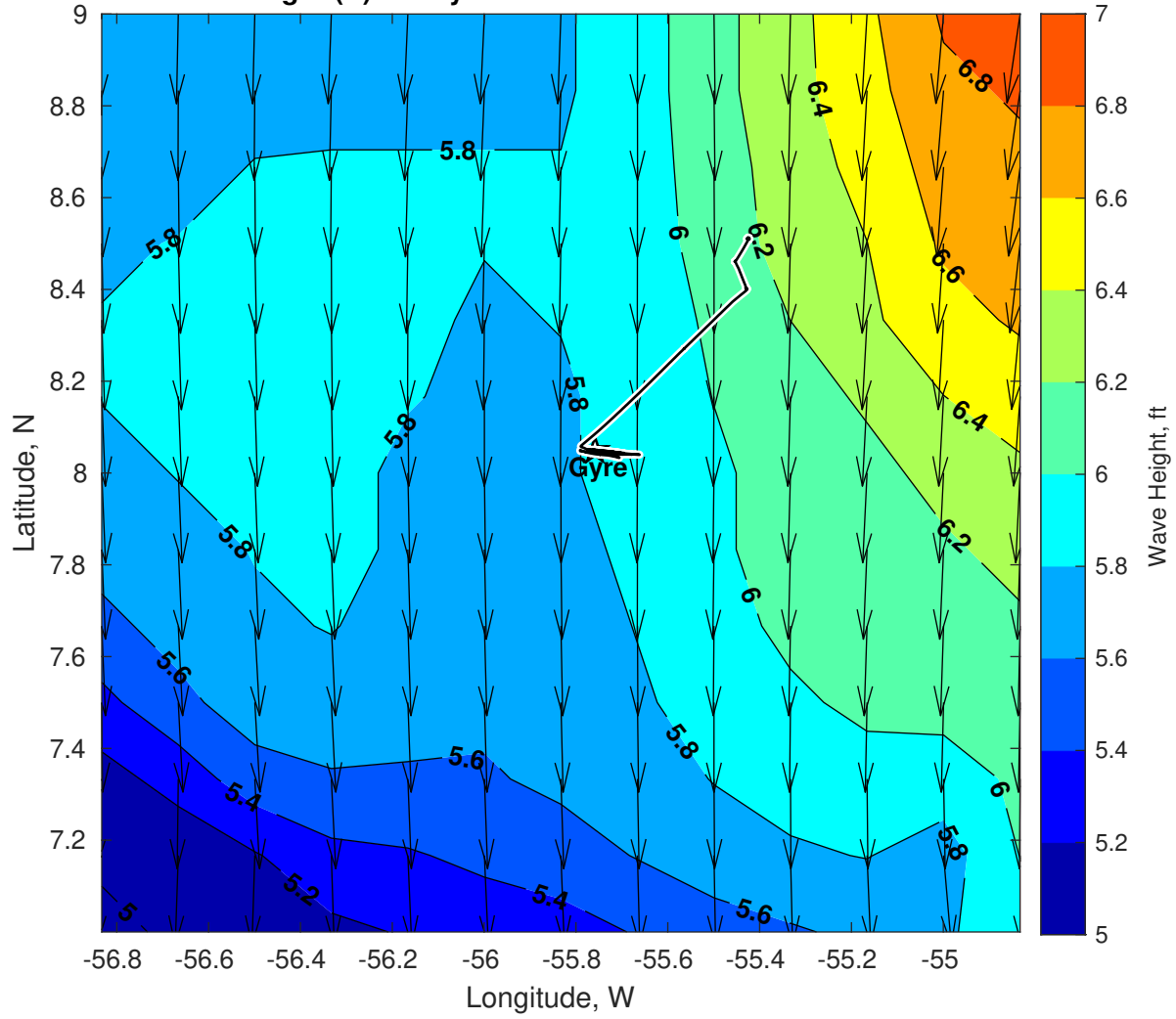
Wave Height (ft) for Gyre at 02-Jan-2025 09:00:00
