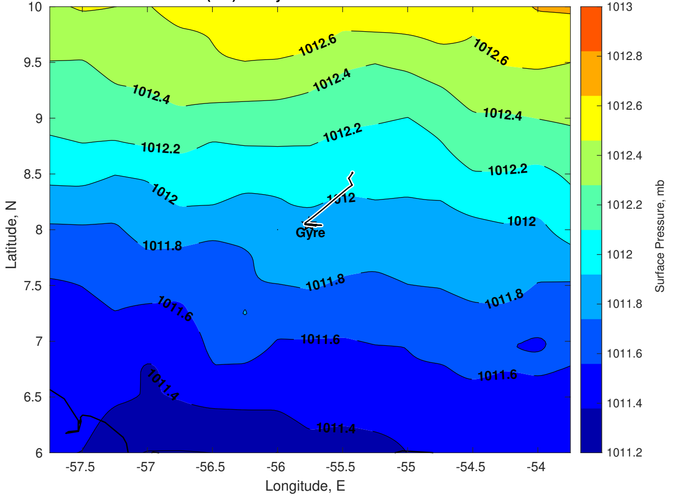
Surface Pressure (mb) for Gyre at 02-Jan-2025 00:00:00
