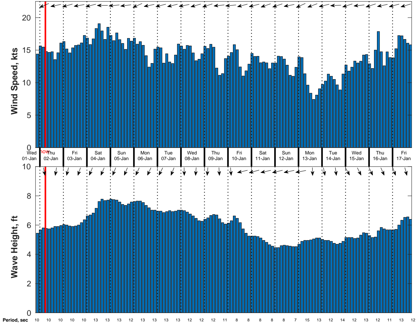
Wind & Wave Forecast for Gyre from 01-Jan-2025 20:00:00 to 17-Jan-2025 20:00:00
