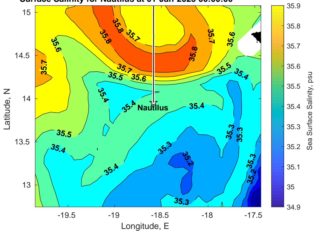
Surface Salinity for Nautilus at 01-Jan-2025 00:00:00
