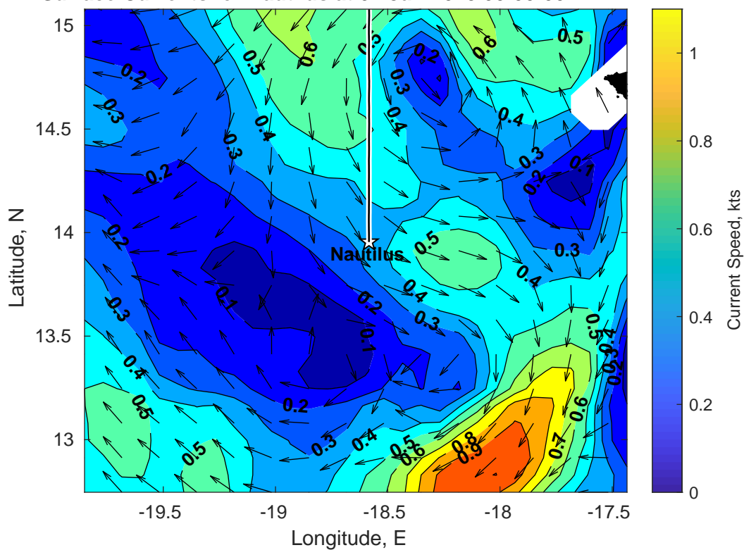
Surface Currents for Nautilus at 01-Jan-2025 00:00:00
