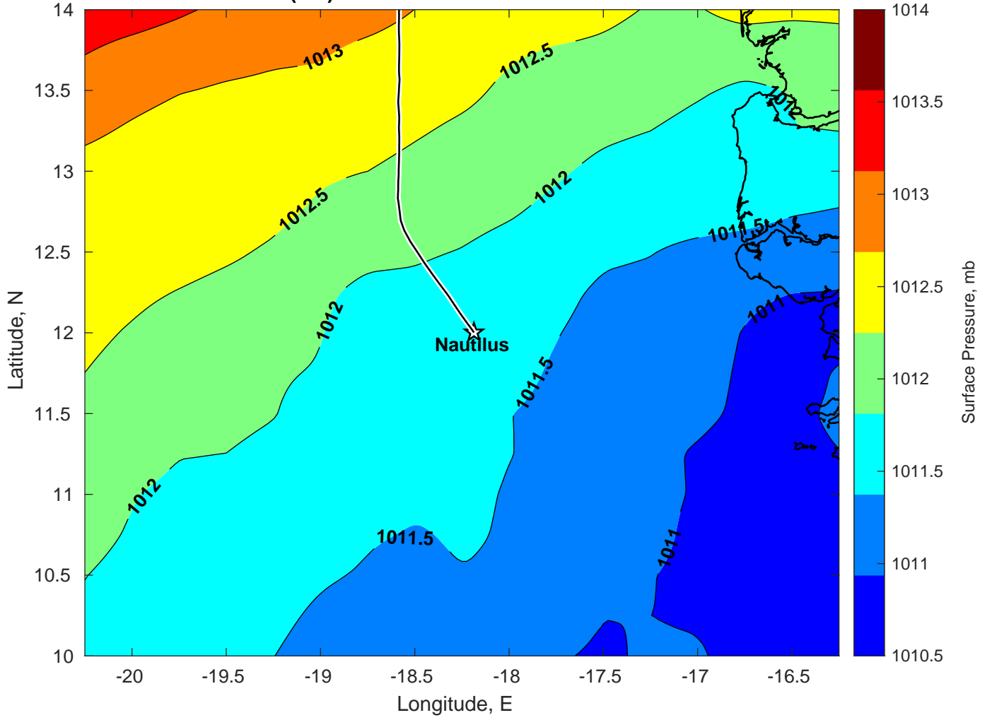
Surface Pressure (mb) for Nautilus at 02-Jan-2025 00:00:00
